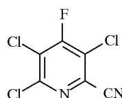
3.6% 4-F-PN
