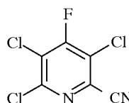
3.6% 4-F-PN
