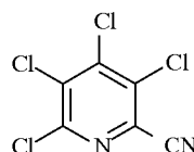
11.2% Cl 4 -PN
