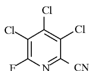
52.6% 6-F-PN
