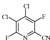
8.0% 3,6-F 2 -PN
