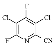
11.3% 4,6-F 2 -PN
