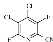
19.0% 3,6-F 2 -PN
