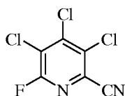
80% 6-F-PN
