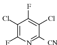
11.3% 4,6-F 2 -PN
