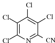
11.2% Cl 4 -PN
