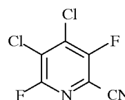
19.0% 3,6-F 2 -PN
