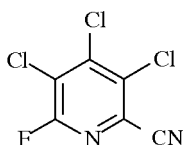
52.6% 6-F-PN
