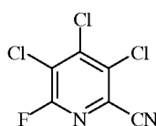
75% 6-F-PN
