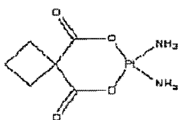
carboplatin
