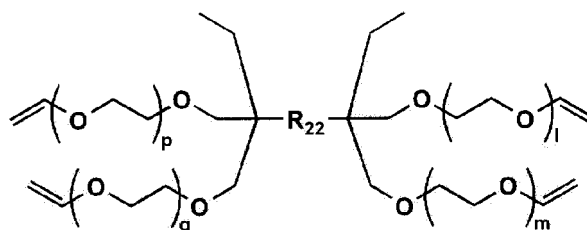
General Formula (5)
