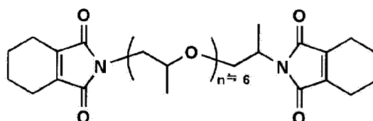
Maleimide Compound 6
