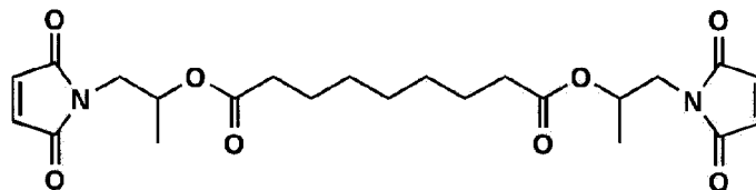
Maleimide Compound 3
