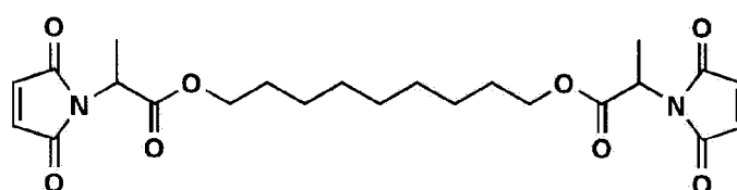
Maleimide Compound 4
