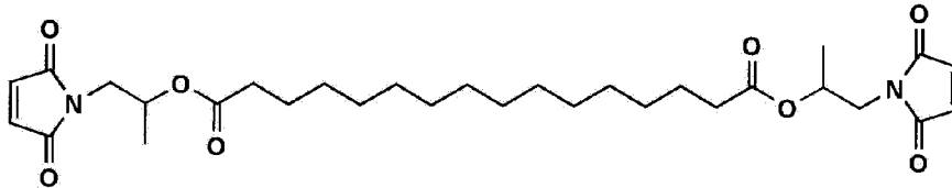
[Chem. 19]
