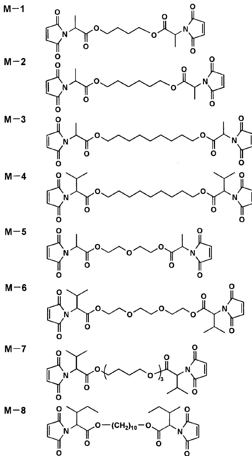
[Chem. 12]
