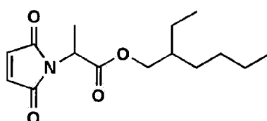
Maleimide Compound 6
