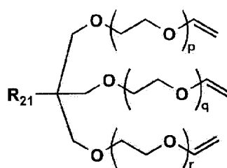
General Formula (4)
