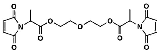
Maleimide Compound 2
