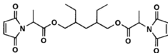
[Chem. 21]
