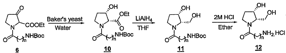
Scheme 2. Synthesis of cis-(-(2R, 3S)-pyrrolidine diol
