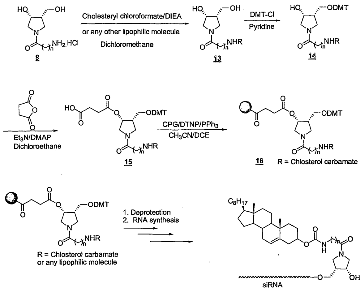
Scheme 3 Synthesis of 3'-conjugated siRNA
