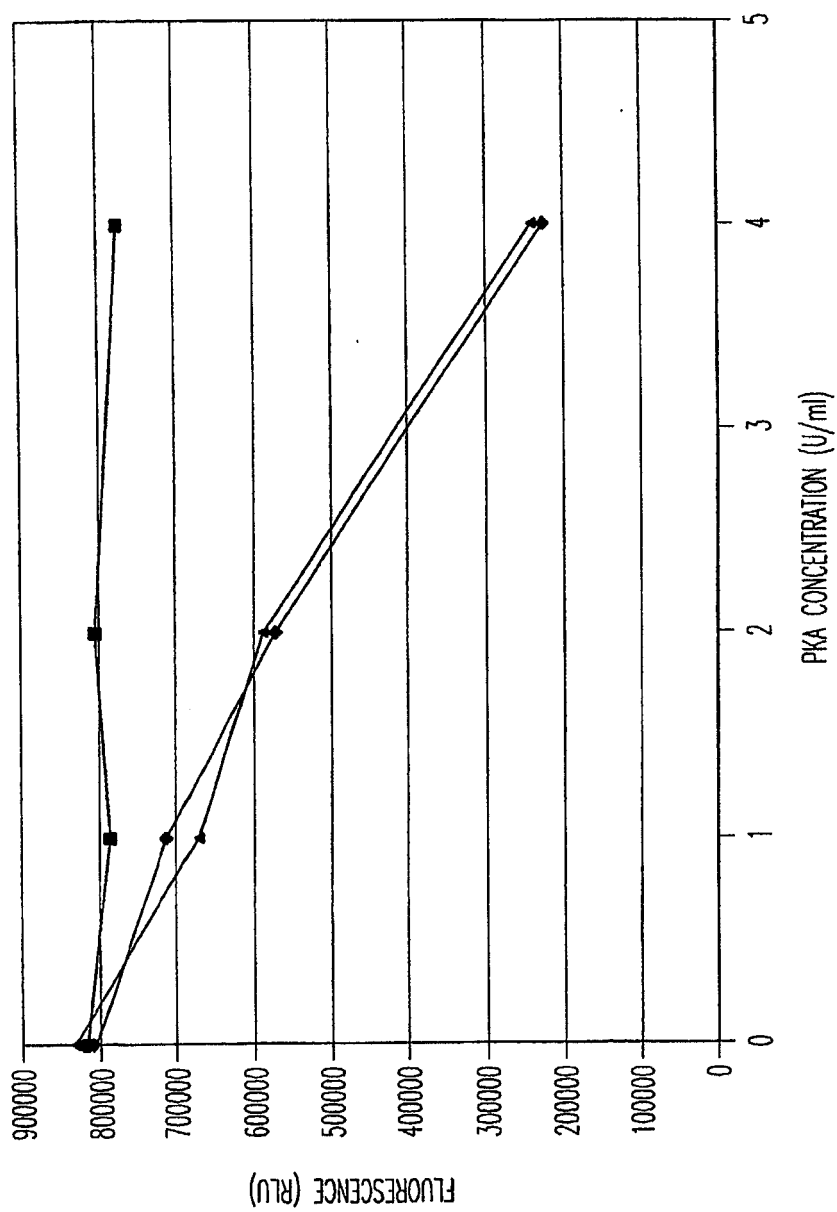
FLUOROGENIC CONTROL ASSAY FOR PKA IN PRESENCE OF CASPASE-3
