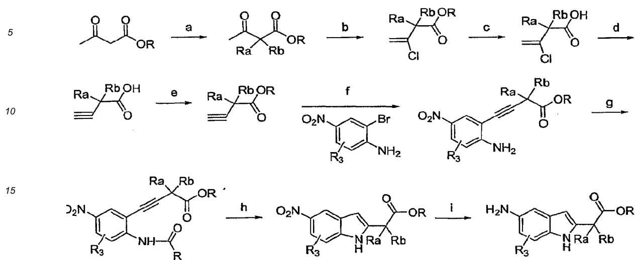
Scheme 31
