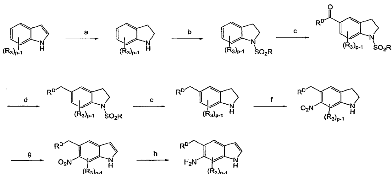
Scheme 14
