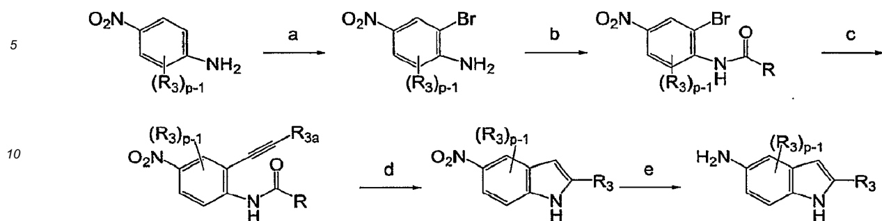
Scheme 17
