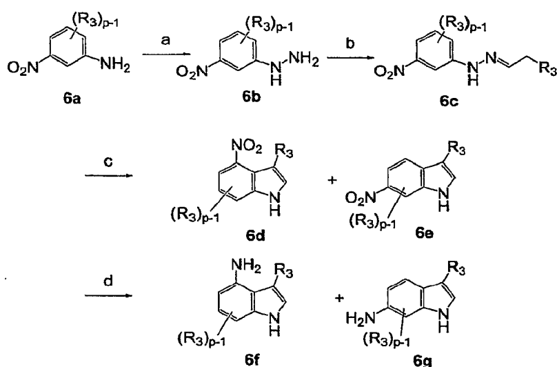
Scheme 6
