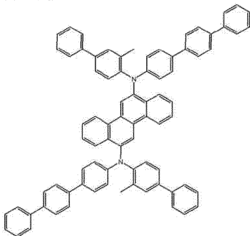
C_{60}H_{36}N_2 Exact Mass: 1046.46 Mol. Wt.: 1047.33 C, 91.74; H, 5.68; N, 2.67
