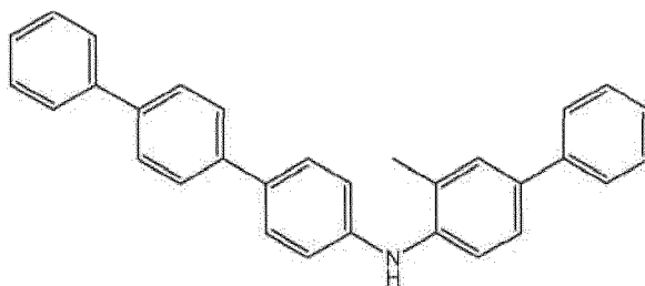
C_{31}H_{25}N Exact Mass: 411.20 Mol. Wt.: 411.54 C, 90.47; H, 6.12; N, 3.40
