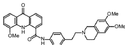
GF120918
