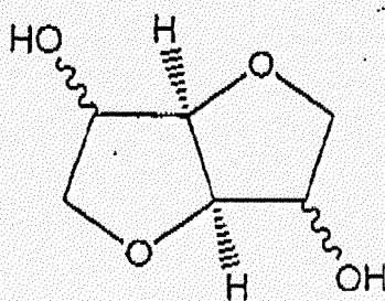
[Chem. 1]
