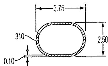
SECTION B-B SCALE 16.000
