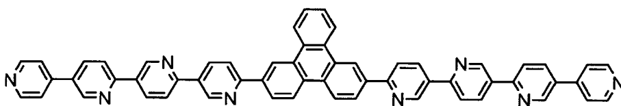
(Compound 48)
