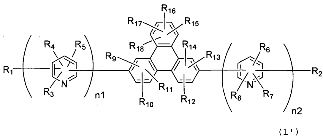
[Chemical Formula 3]
