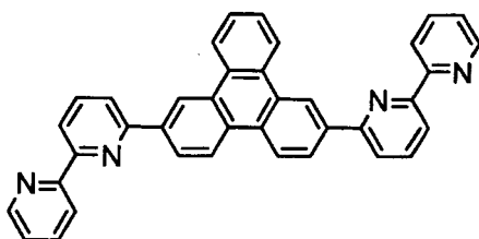
[Chemical Formula 9]
