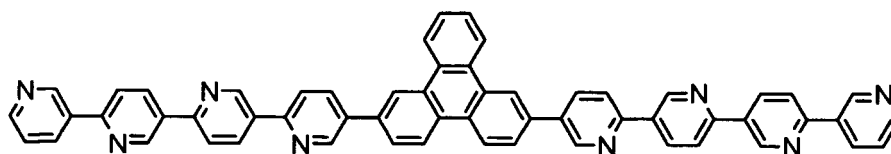
(Compound 46)
