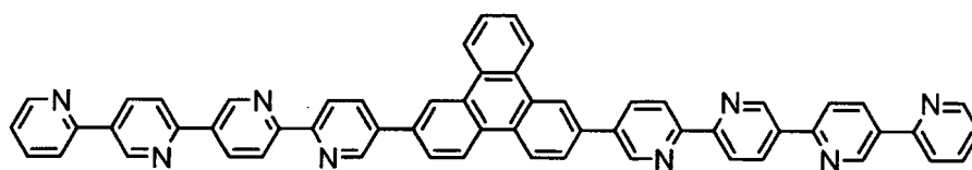
(Compound 44)
