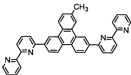
[Chemical Formula 11]
