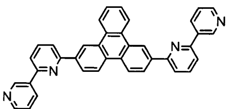
[Chemical Formula 13]
