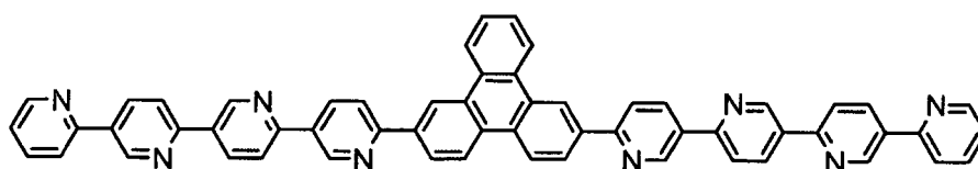
(Compound 47)
