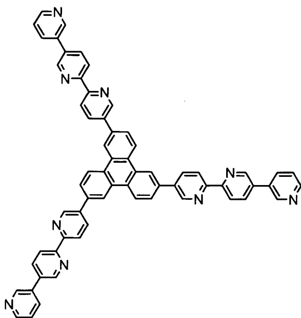
[Chemical Formula 46]
