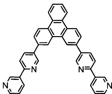
[Chemical Formula 18]
