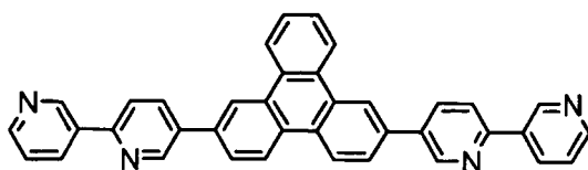
[Chemical Formula 12]
