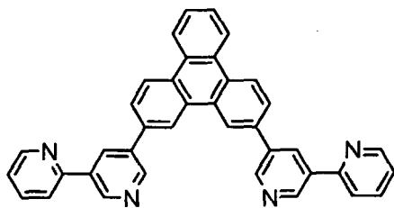
[Chemical Formula 21]
