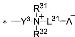
(a3-1)
