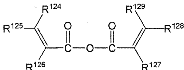
Formula (b-2)
