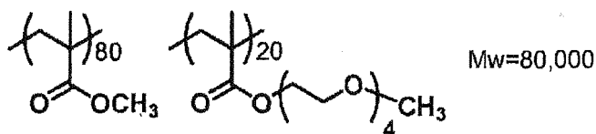
Binder polymer (3)
