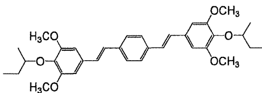
Sensitizing dye (3)
