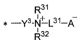
(a3-1)
