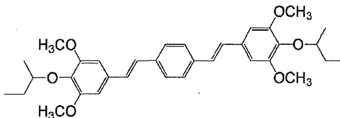
Sensitizing dye (3)
