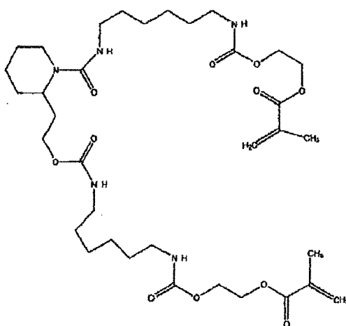
Polymerization compound (2)
