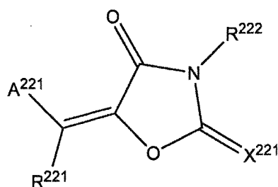
Formula (IX)
