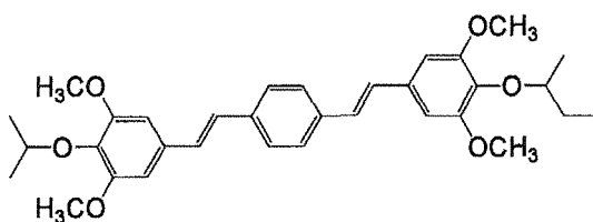
Sensitizing dye (2)
