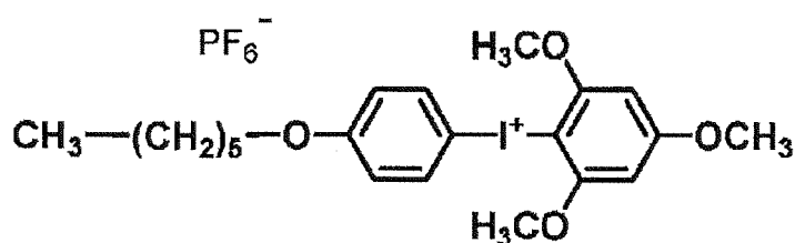
Polymerization initiator (3)
