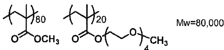
Binder polymer (3)
