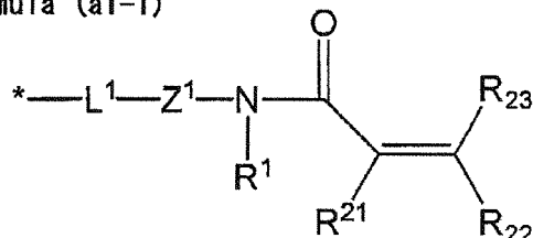
Formula (a1-1)
