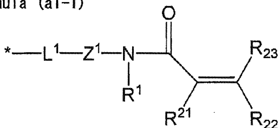
Formula (a1-1)
