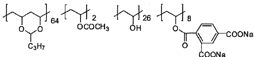
Binder polymer (2) (acid value = 66 mgKOH/g)
