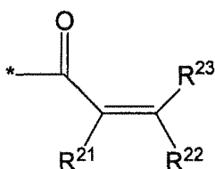
Formula (Q)
