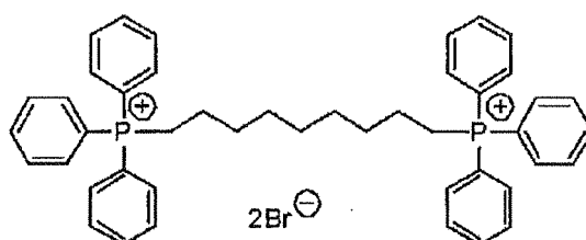
Oil-sensitizer (1)
