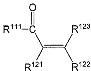
Formula (b-1)
