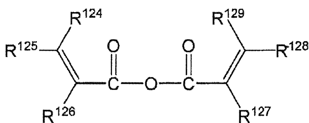
Formula (b-2)
