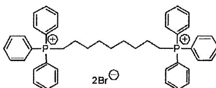
Oil-sensitizer (1)
