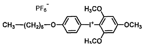
Polymerization initiator (3)
