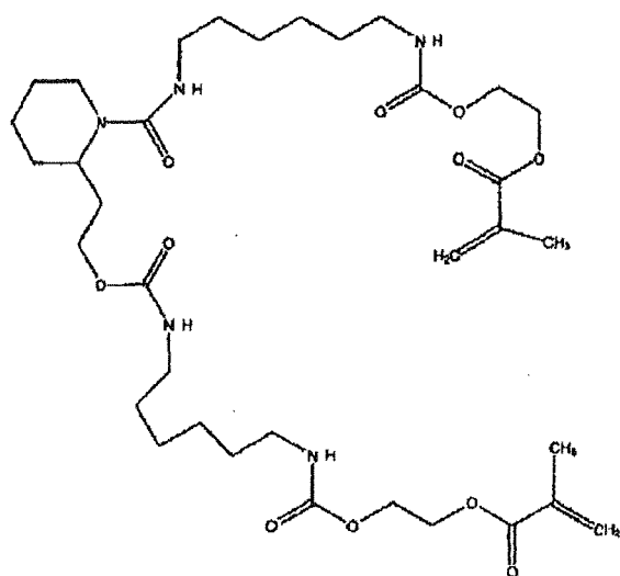
Polymerization compound (2)
