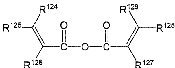
Formula (b-2)
