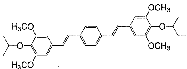
Sensitizing dye (2)
