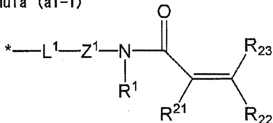
Formula (a1-1)
