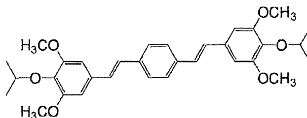
Sensitizing dye (4)
