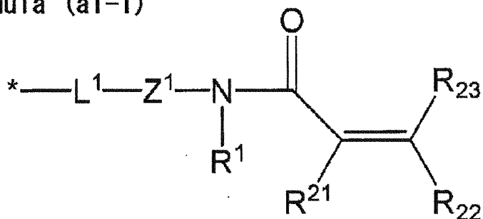
Formula (a1-1)
