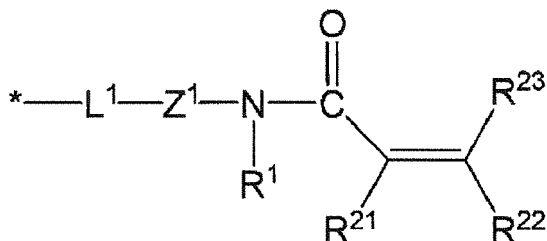
Formula (a1-1)
