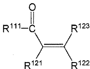
Formula (b-1)
