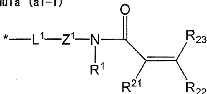
Formula (a1-1)
