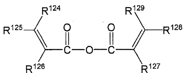
Formula (b-2)
