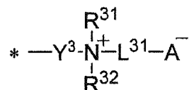
(a3-1)
