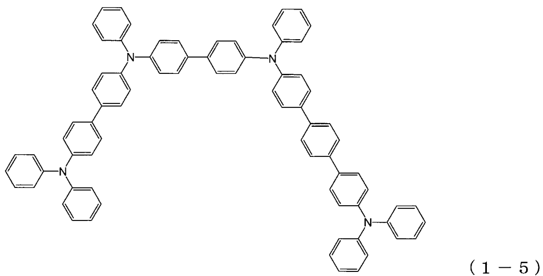
[Chemical 19]
