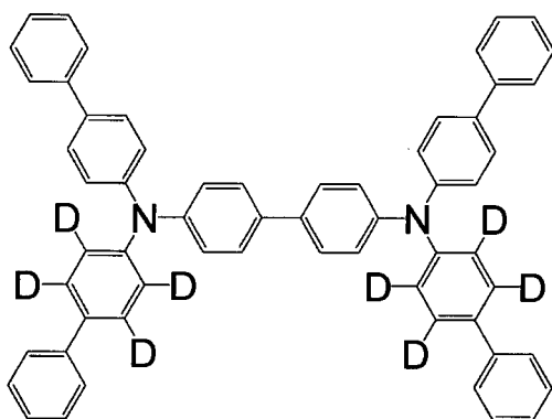
[Chemical 55]
