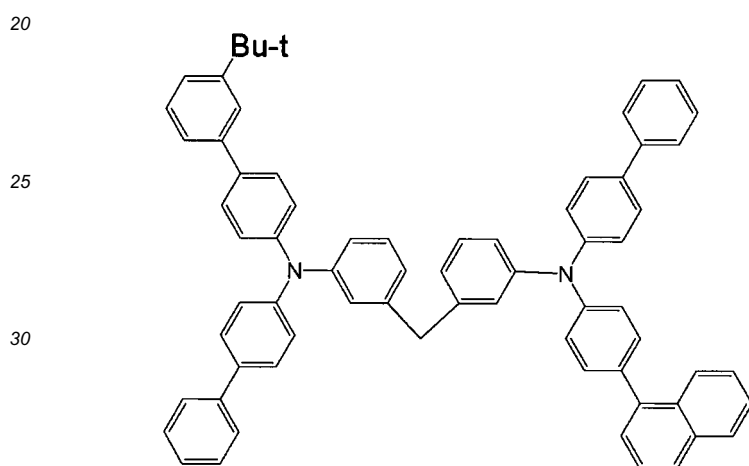
[Chemical 47]
