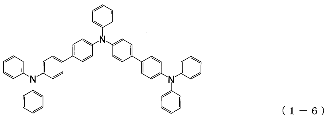
[Chemical 19]
