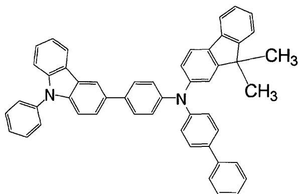
[Chemical 62]
