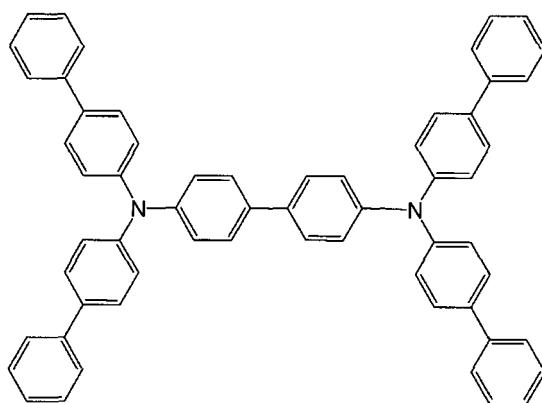
[Chemical 35]
