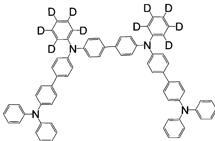
[Chemical 67]
