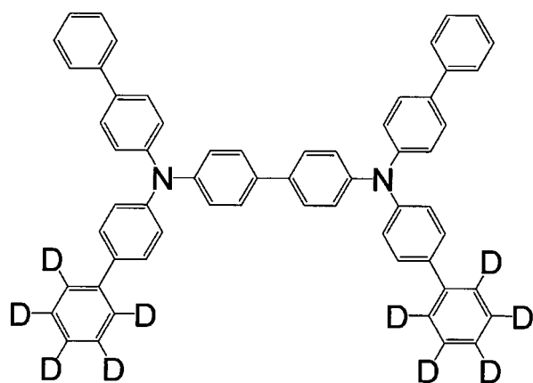
[Chemical 56]
