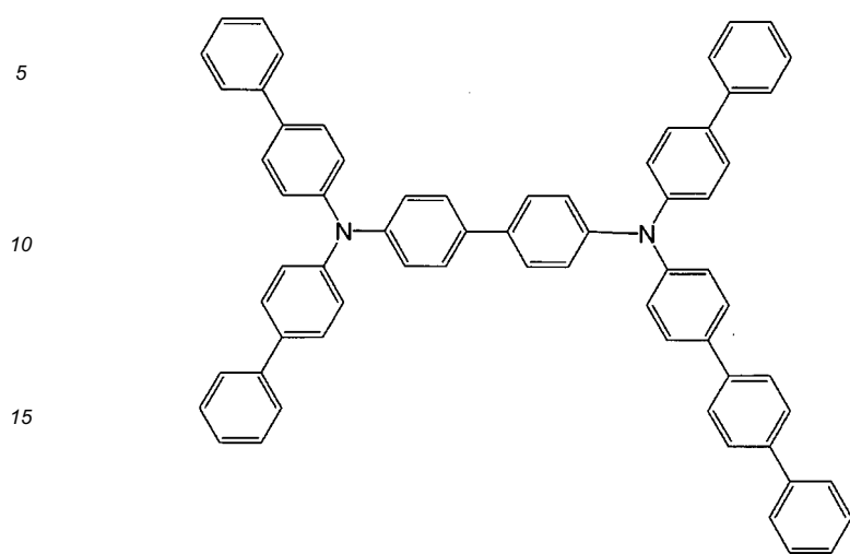
[Chemical 37]
