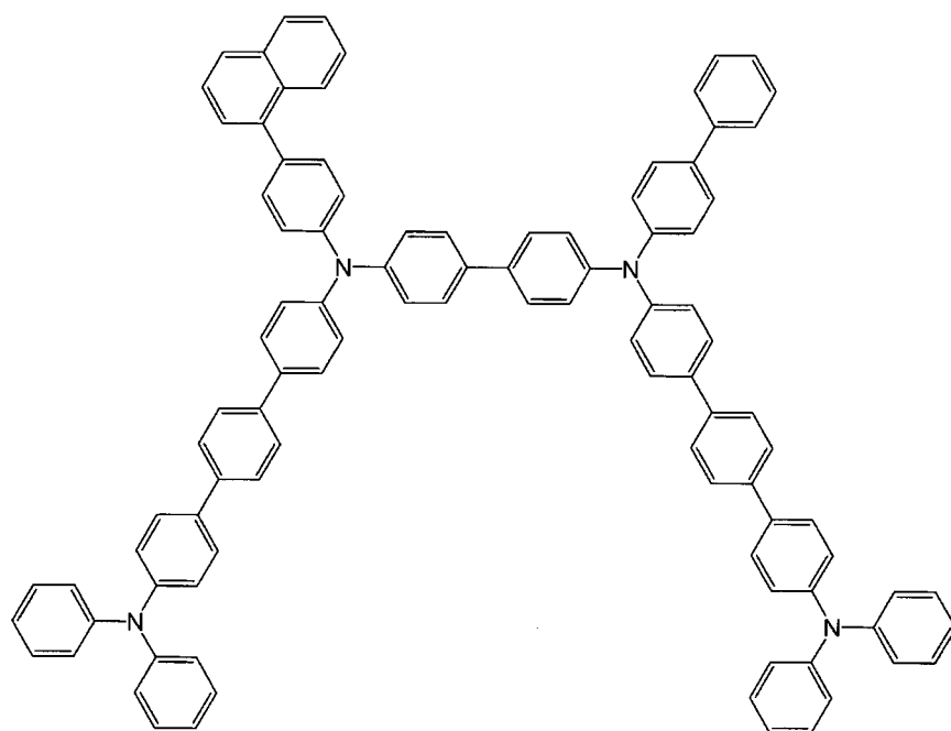
[Chemical 20]
