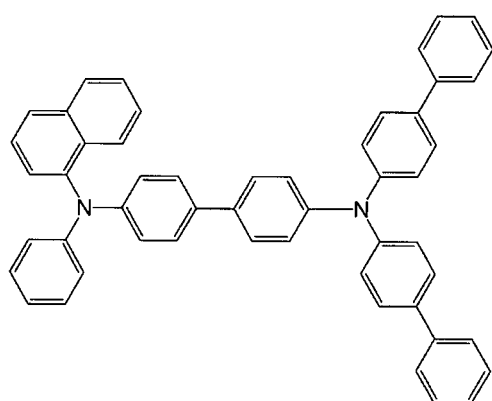
[Chemical 50]
