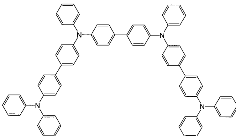
[Chemical 14]
