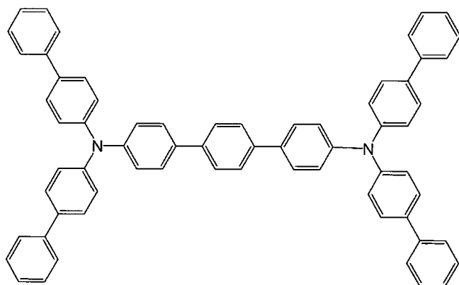
[Chemical 40]
