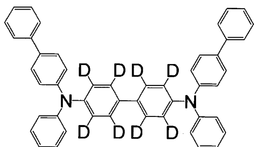
[Chemical 54]
