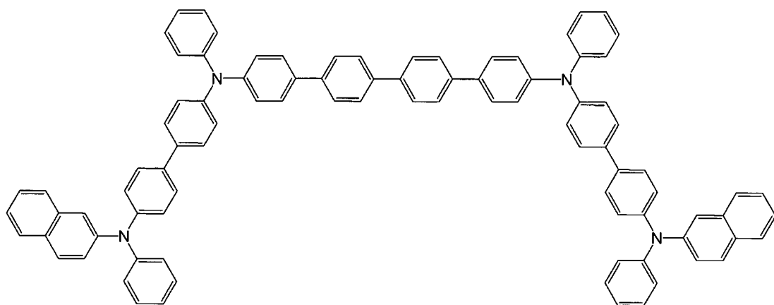
[Chemical 22]
