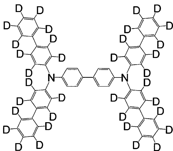
[Chemical 59]
