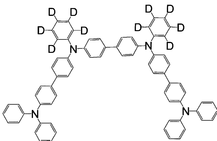
[Chemical 29]
