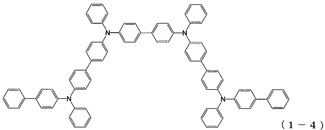
[Chemical 17]
