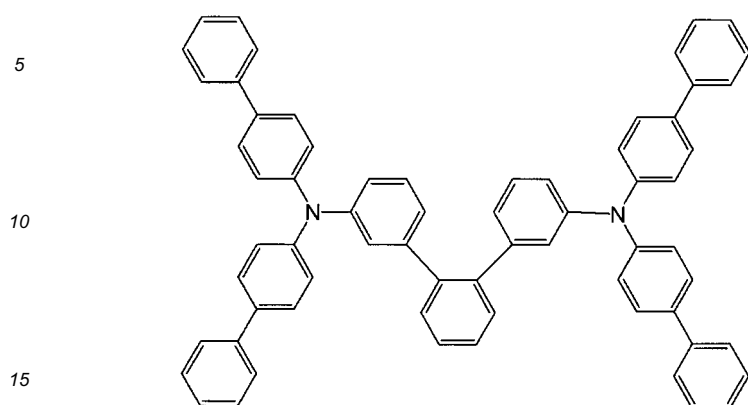
[Chemical 42]
