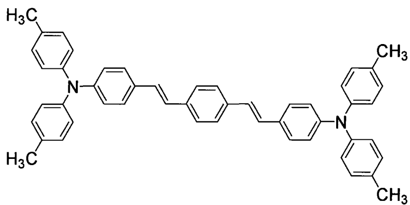
[Chemical 65]
