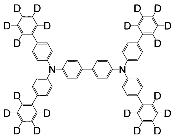
[Chemical 58]
