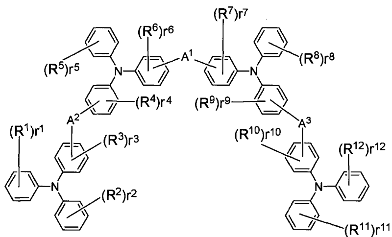
[Chemical 1]
