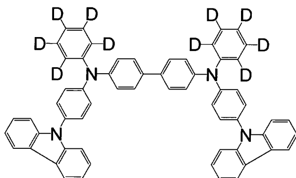
[Chemical 28]
