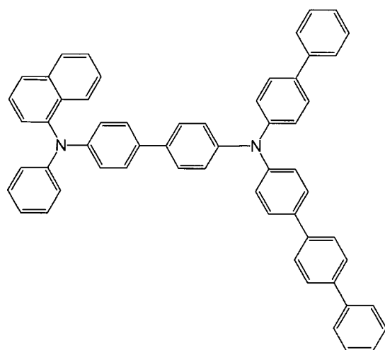
[Chemical 51]
