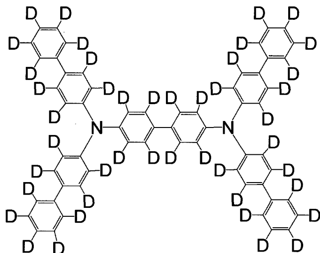
[Chemical 60]
