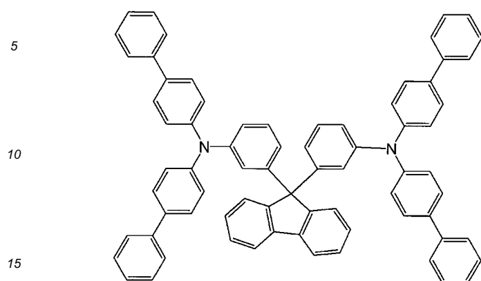
[Chemical 46]
