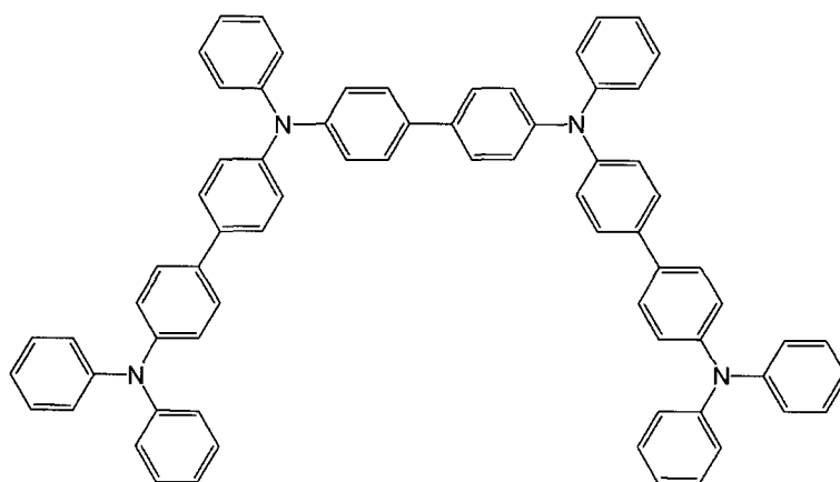
[Chemical 63]
