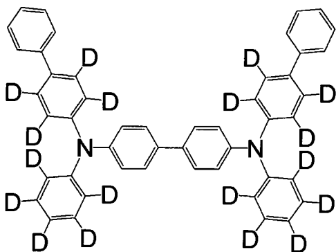
[Chemical 55]
