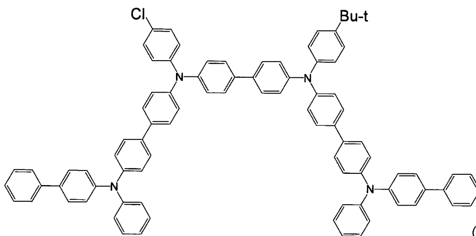
[Chemical 21]
