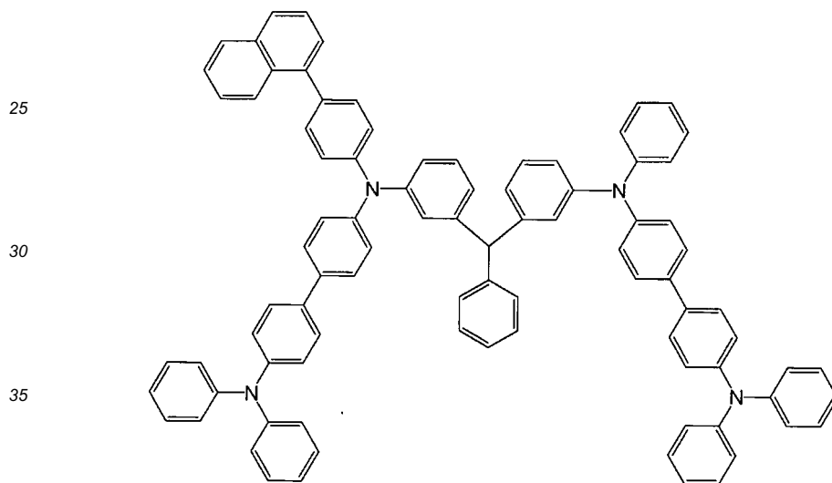
[Chemical 26]
