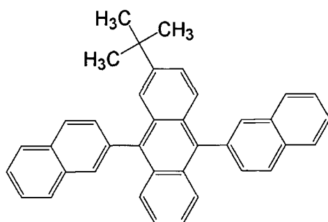
[Chemical 66]
