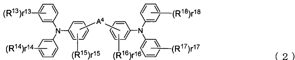
[Chemical 34]
