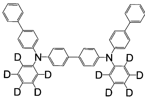
[Chemical 53]
