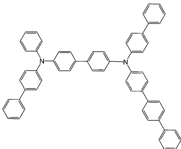
[Chemical 39]
