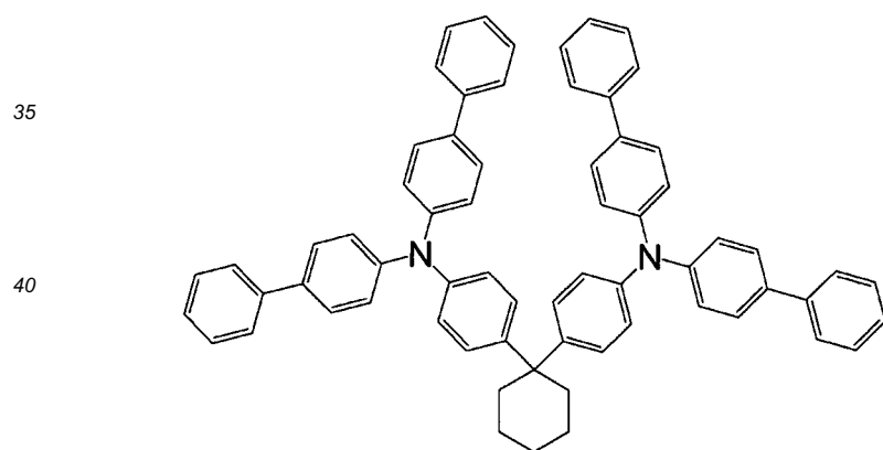
[Chemical 44]
