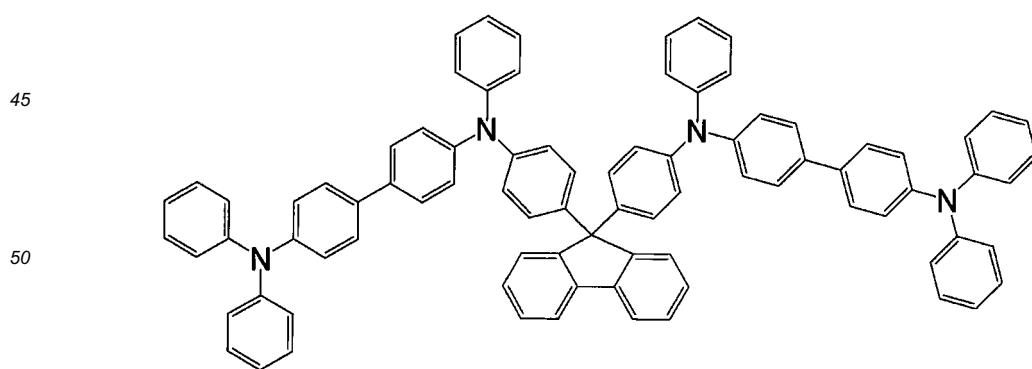
[Chemical 27]
