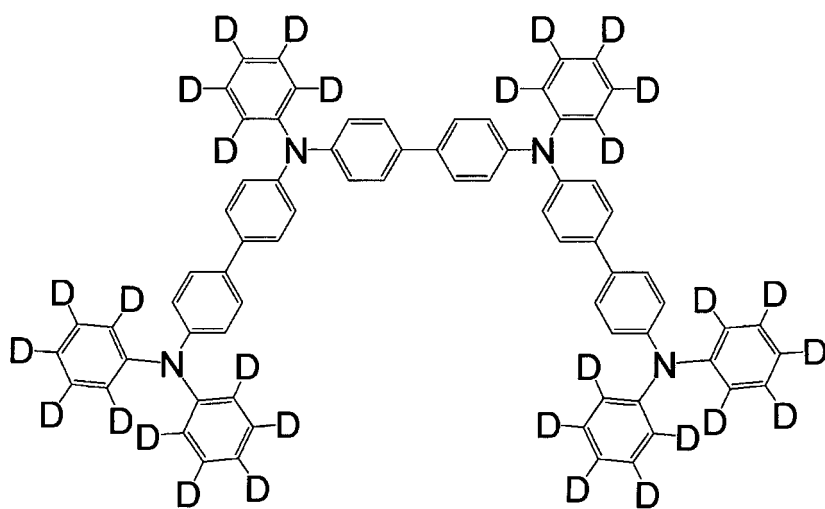
[Chemical 32]
