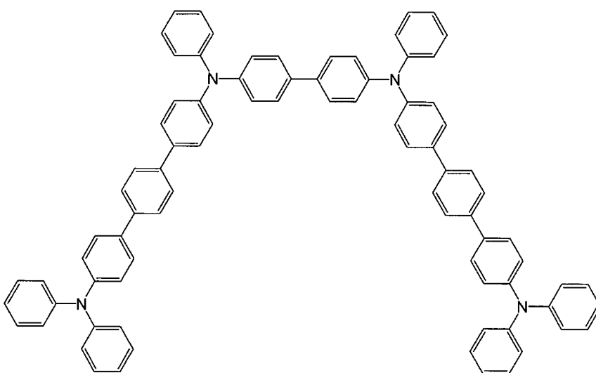
[Chemical 16]
