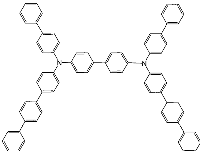
[Chemical 36]
