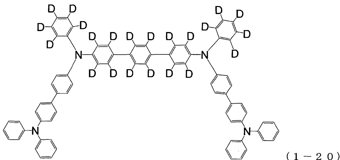
[Chemical 33]
