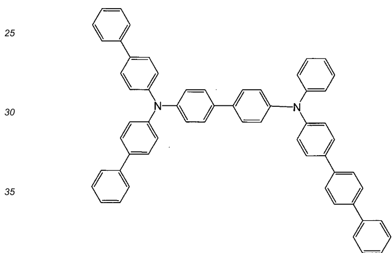
[Chemical 38]
