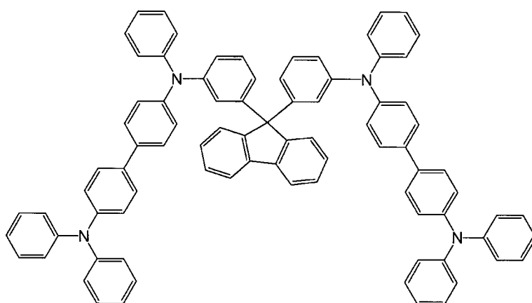
[Chemical 24]
