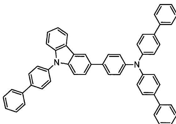
[Chemical 61]
