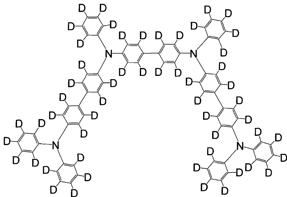
[Chemical 32]
