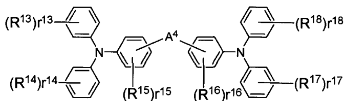
[Chemical 7]
