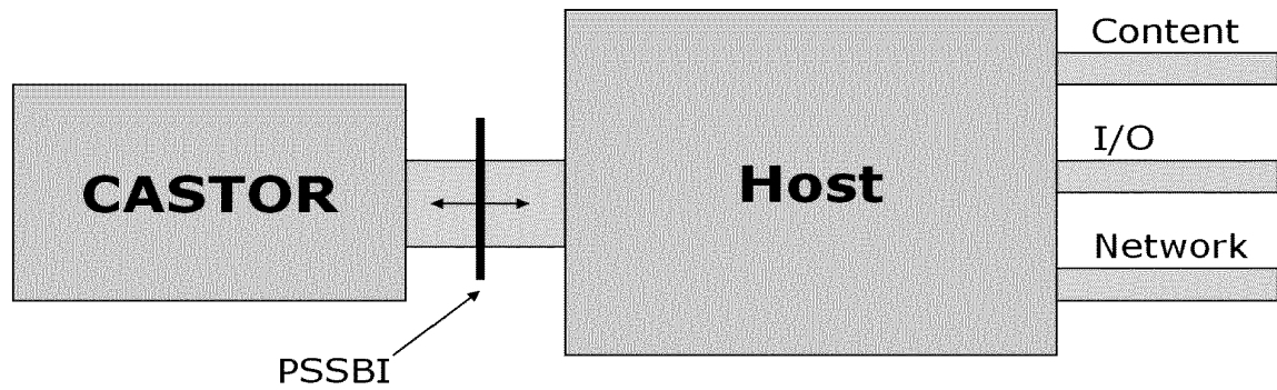
Figure 6: The PSSBI approach as API-filter.
