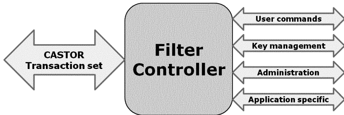
Figure 7: Logical PSSBI filter interface functionality.
