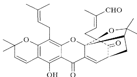
Gh-2501 (isomorellin)
