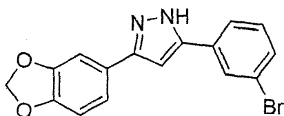
5-(3-Bromophenyl)-3-(3,4-methylenedioxyphenyl)pyrazole
