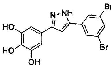
5-(3,5-Dibromophenyl)-3-(3,4,5-trihydroxyphenyl)pyrazole (anle 145d)
