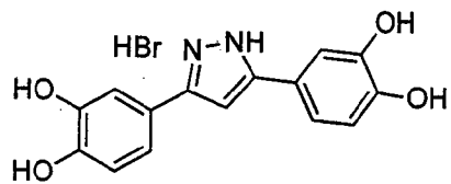
sery159a C_{15}H_{13}BrN_2O_4 Mol. Wt.: 365,18
