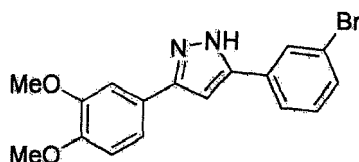
5-(3-Bromophenyl)-3-(3,4-dimethoxyphenyl)pyrazole (sery255b)
