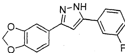
5-(3-Bromophenyl)-3-(3,4-methylenedioxyphenyl)pyrazole
