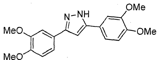
3,5-Bis(3,4-dimethoxyphenyl)pyrazole
