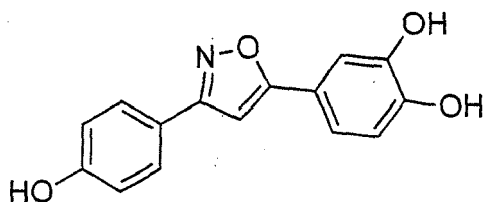
3-(4-Hydroxyphenyl)-5-(3,4-dihydroxyphenyl)isoxazole
