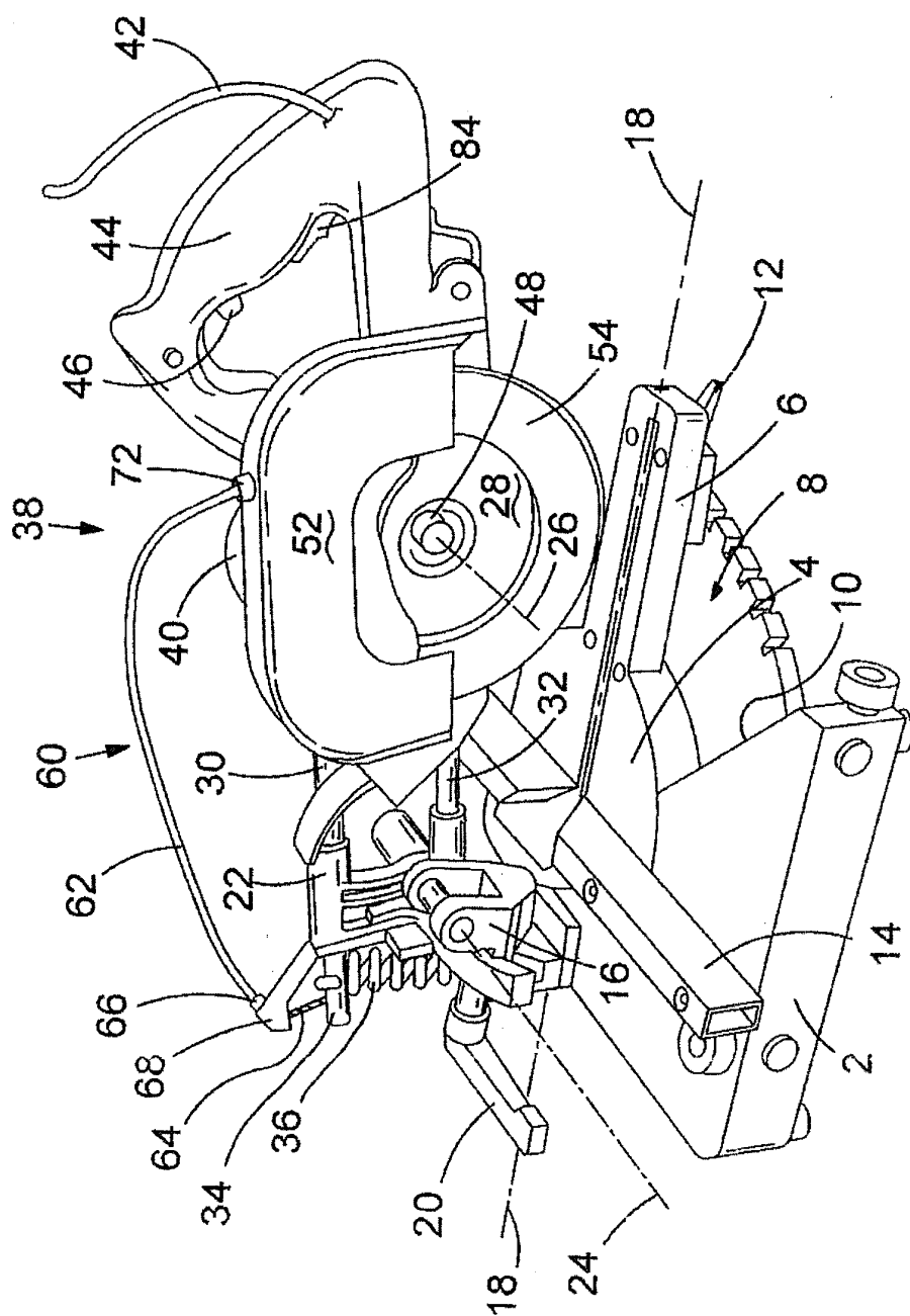
FIG. 1 (PRIOR ART)
