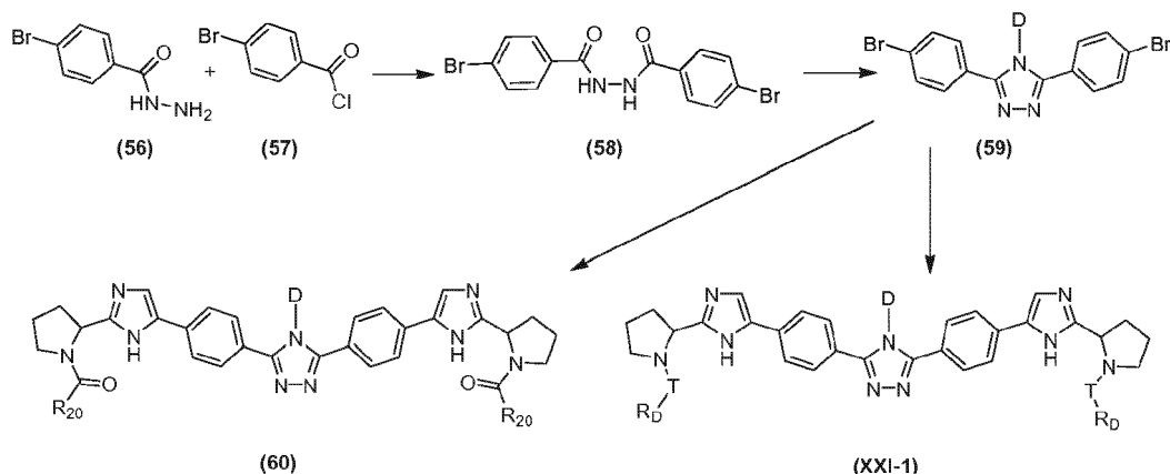
Scheme XXI
