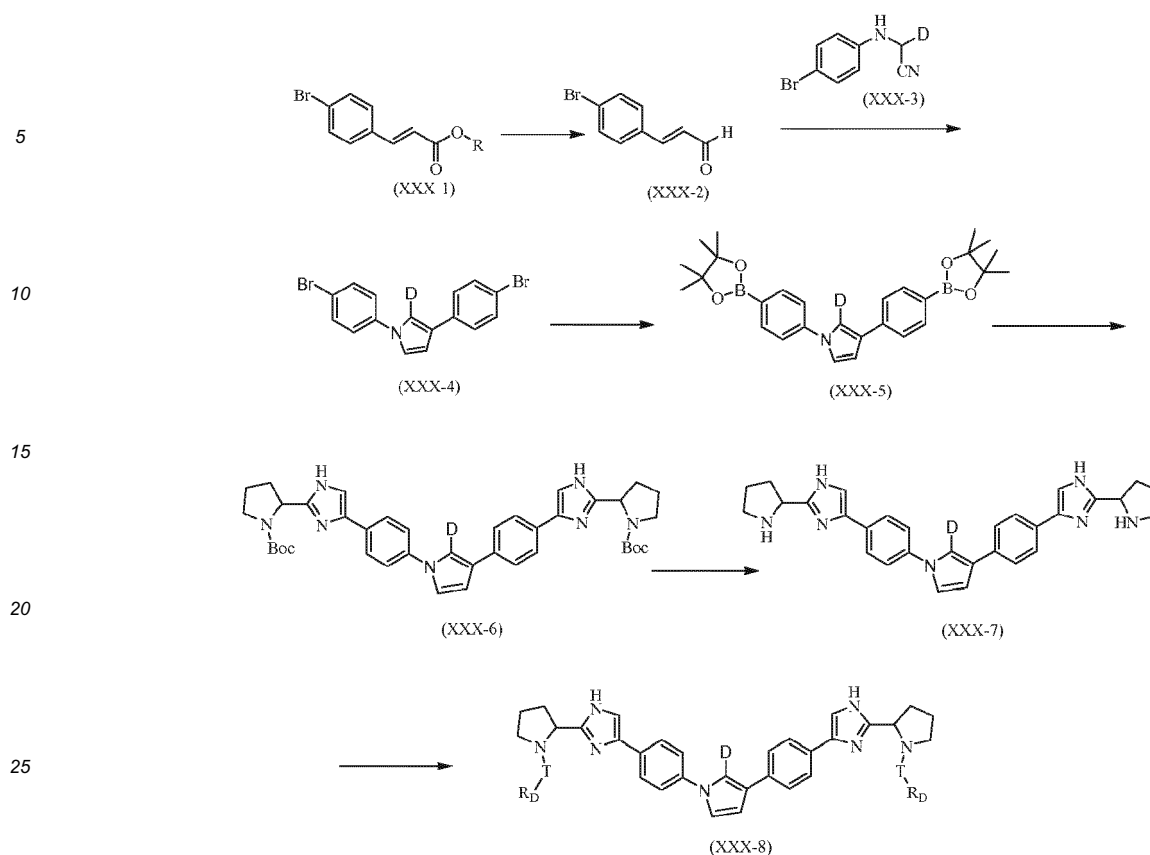
Scheme XXX
