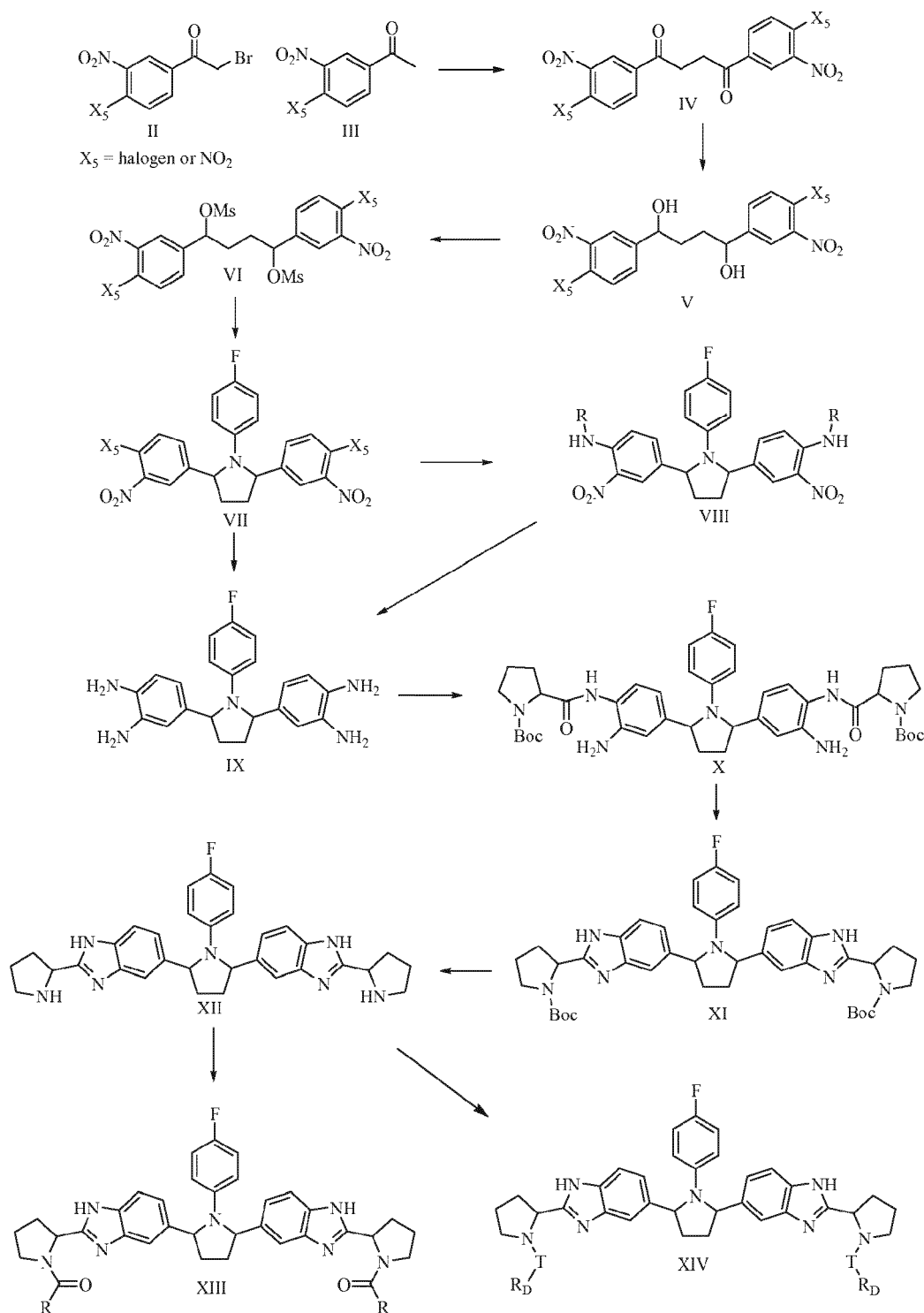
Scheme IV
