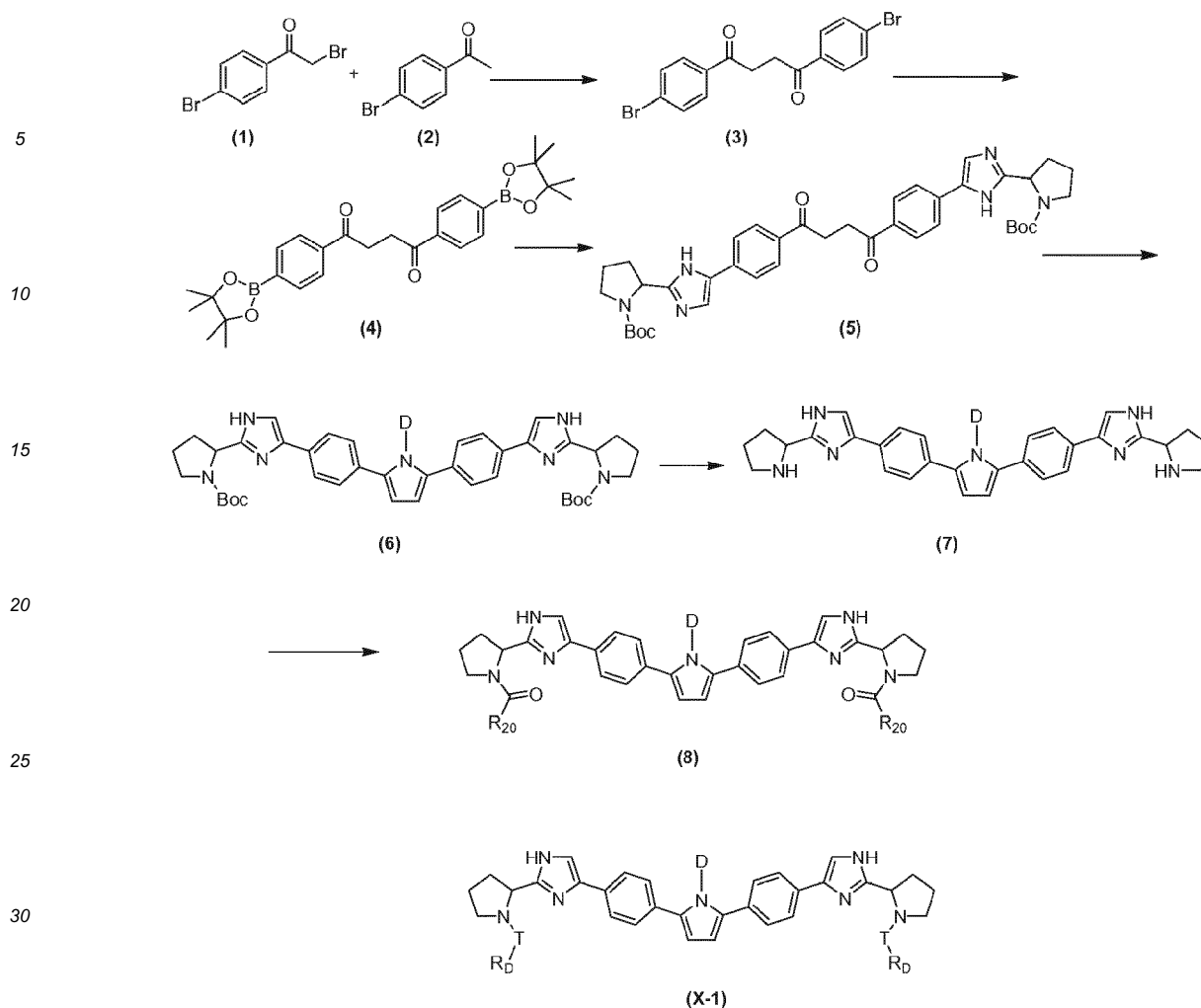
Scheme X
