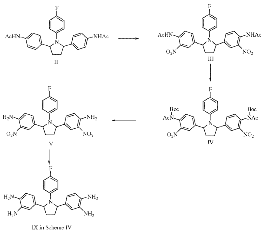
Scheme V
