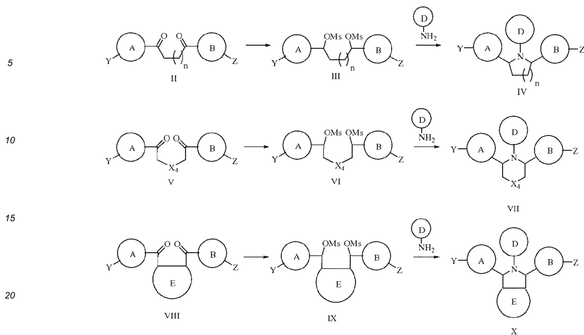
Scheme I
