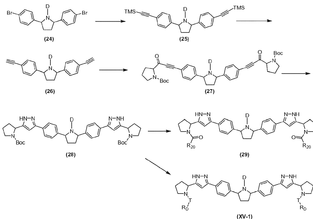
Scheme XV
