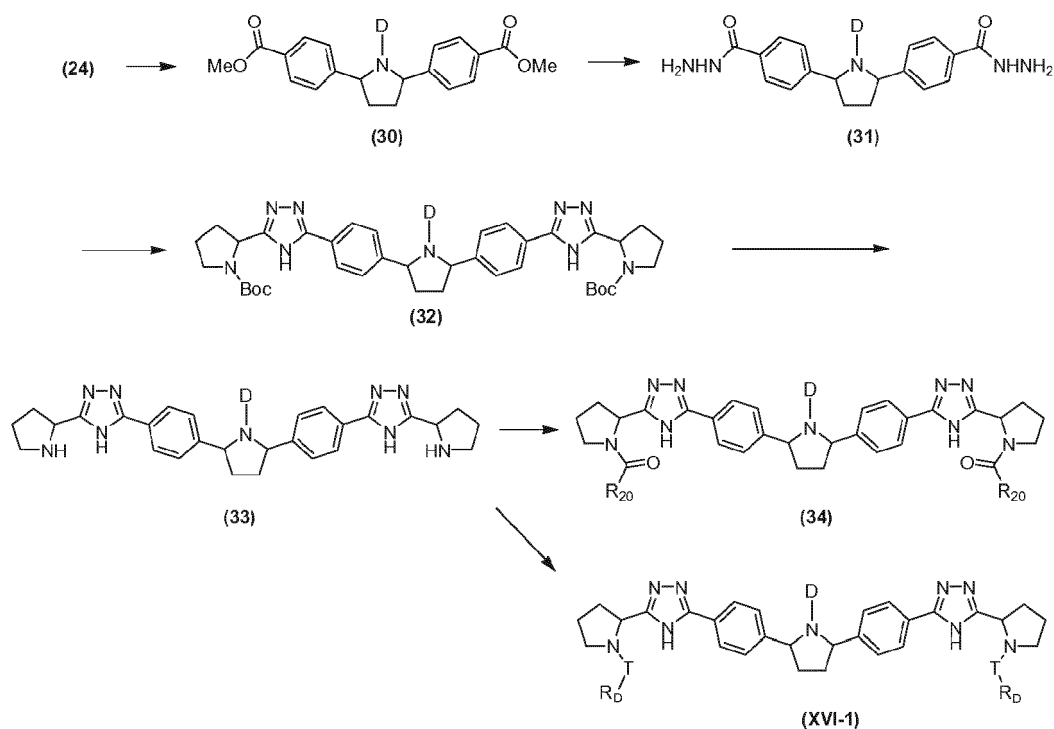
Scheme XVI
