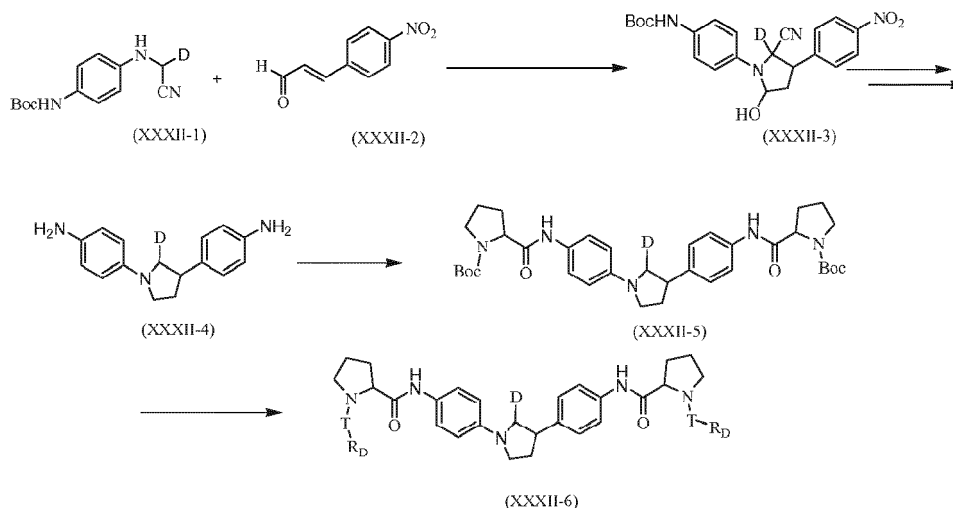
Scheme XXXII
