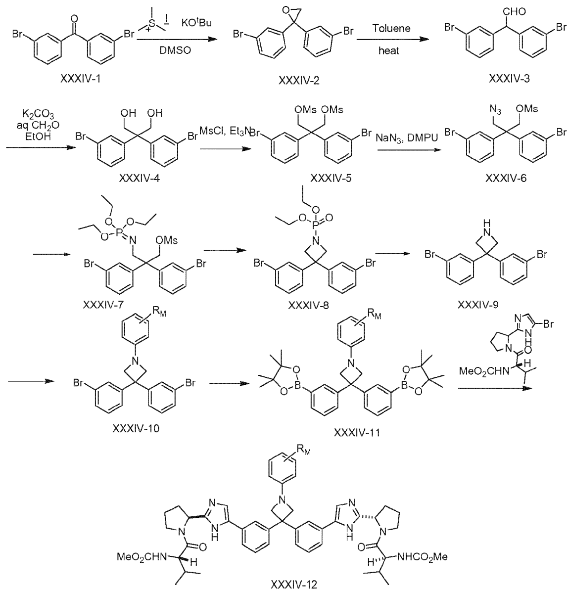
Scheme XXXIV
