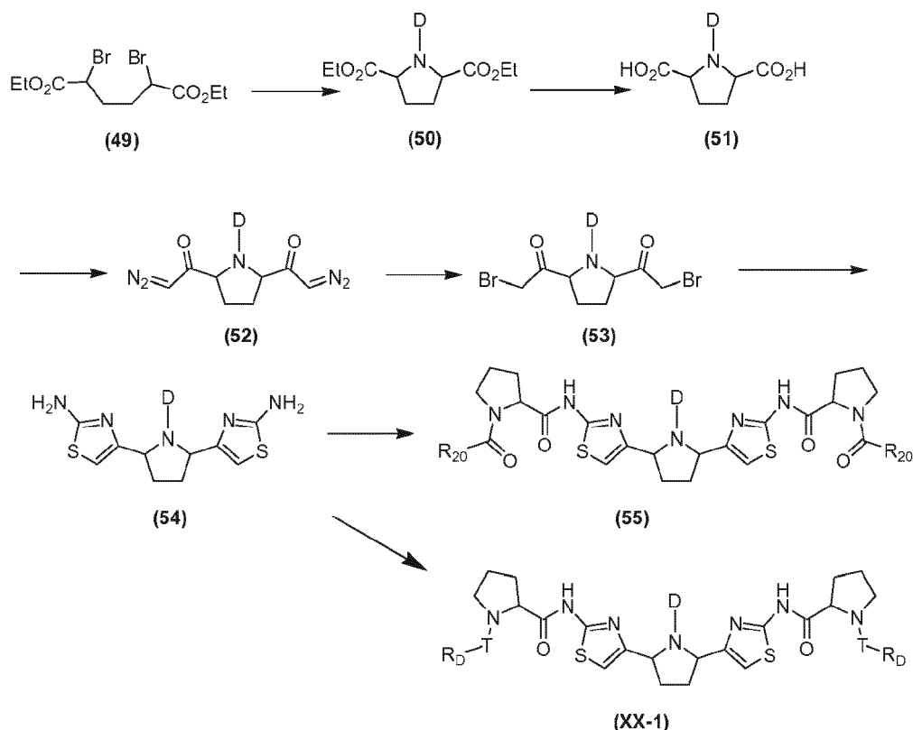
Scheme XX
