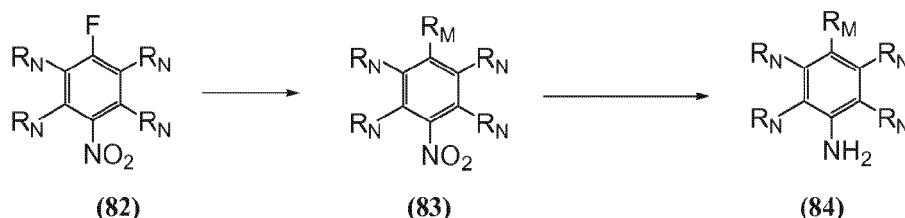
Scheme XXV
