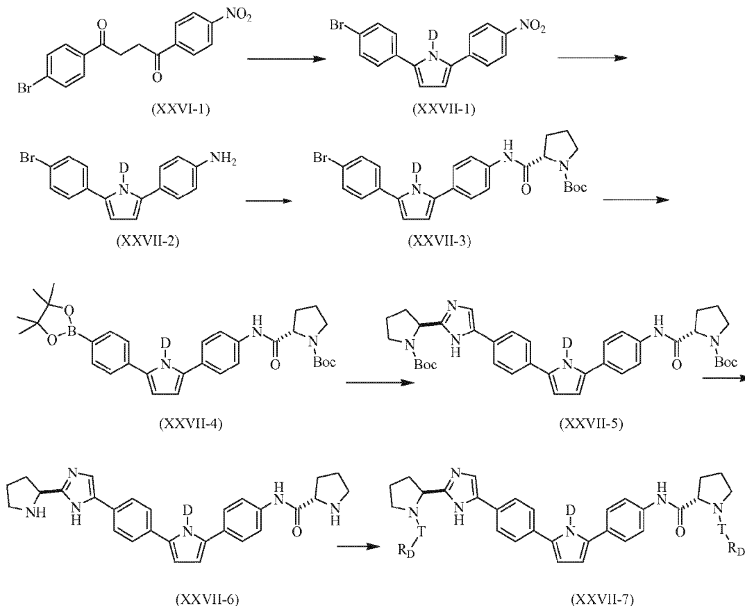
Scheme XXVII
