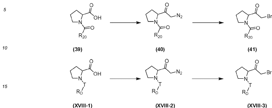
Scheme XVIII
