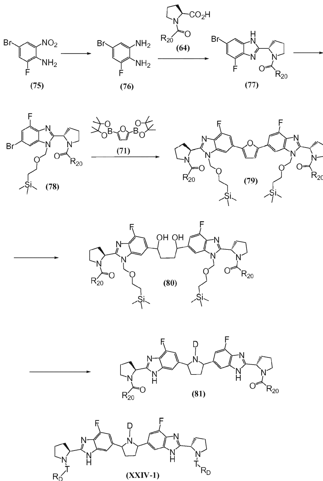
Scheme XXIV
