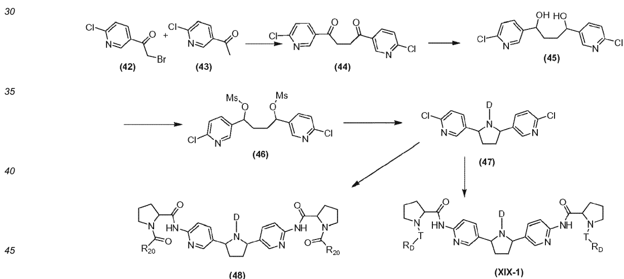
Scheme XIX
