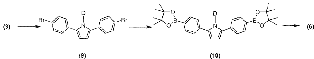
Scheme XI
