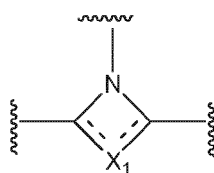
X-1
