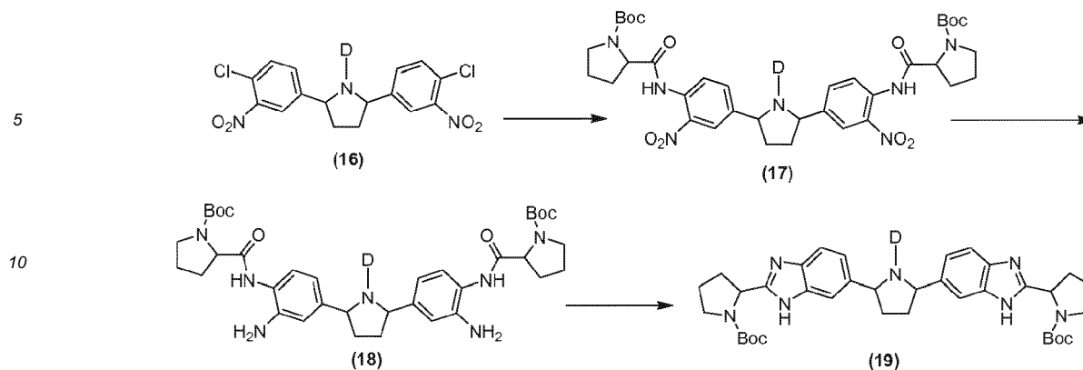
Scheme XIII
