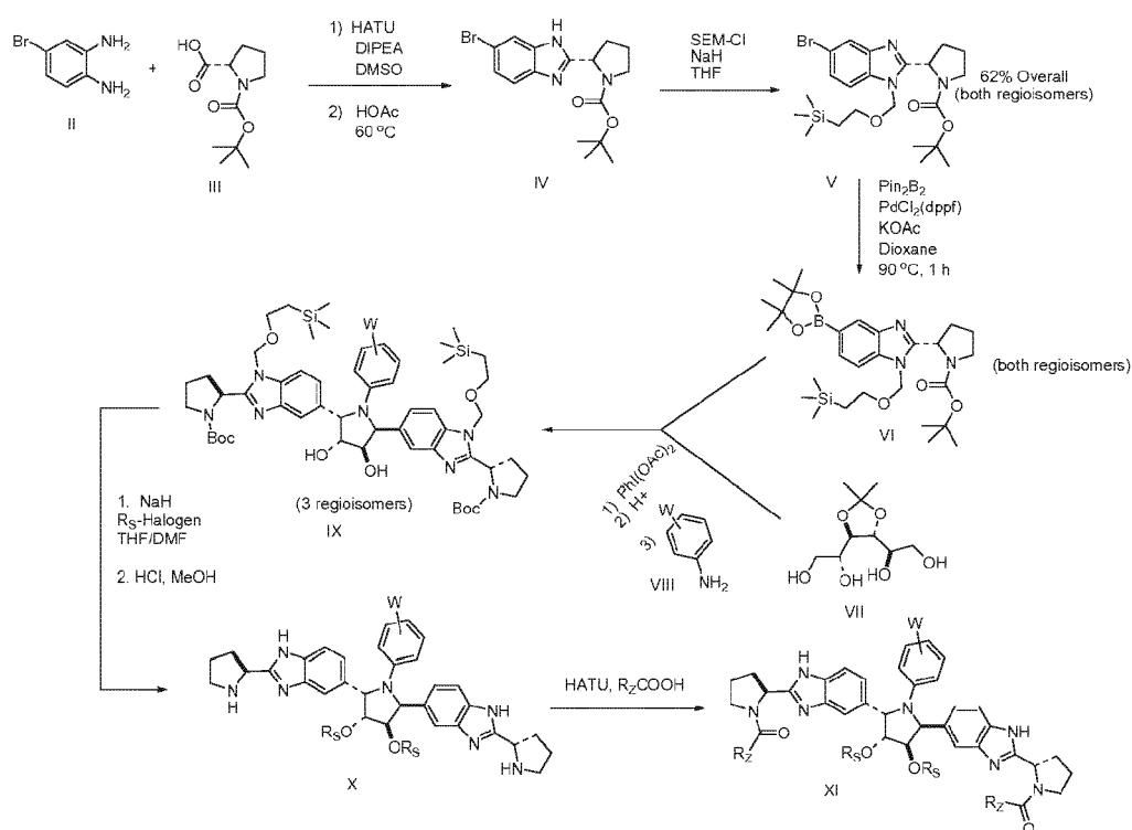
Scheme IX
