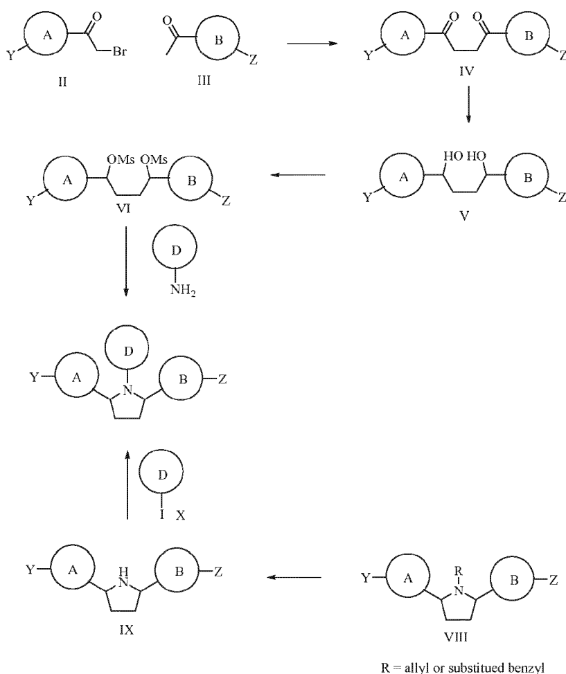
Scheme III
