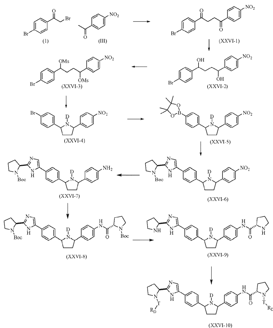
Scheme XXVI
