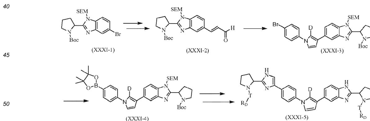
Scheme XXXI
