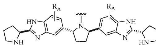
11-2
