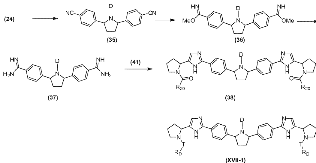
Scheme XVII
