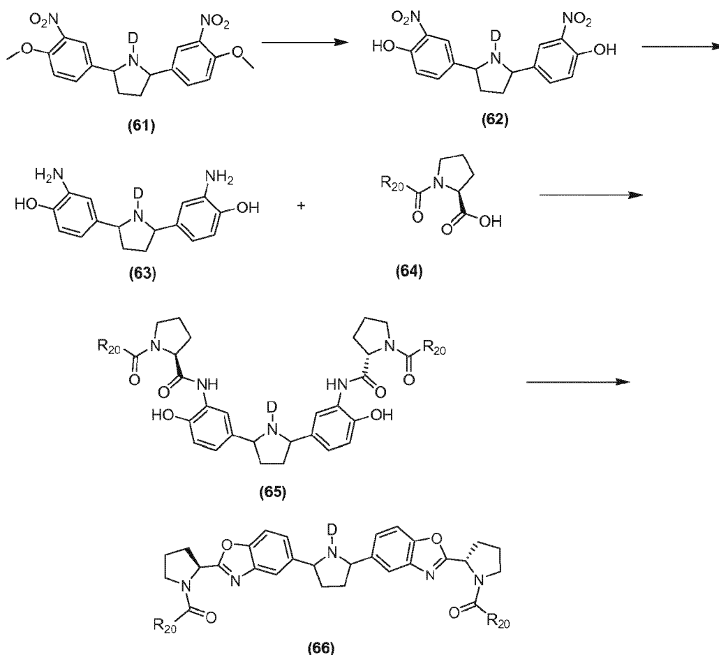
Scheme XXII
