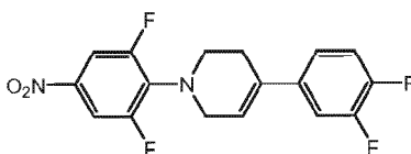
1-(2,6-difluoro-4-nitrophenyl)-4-(3,4-difluorophenyl)-1,2,3,6-tetrahydropyridine
