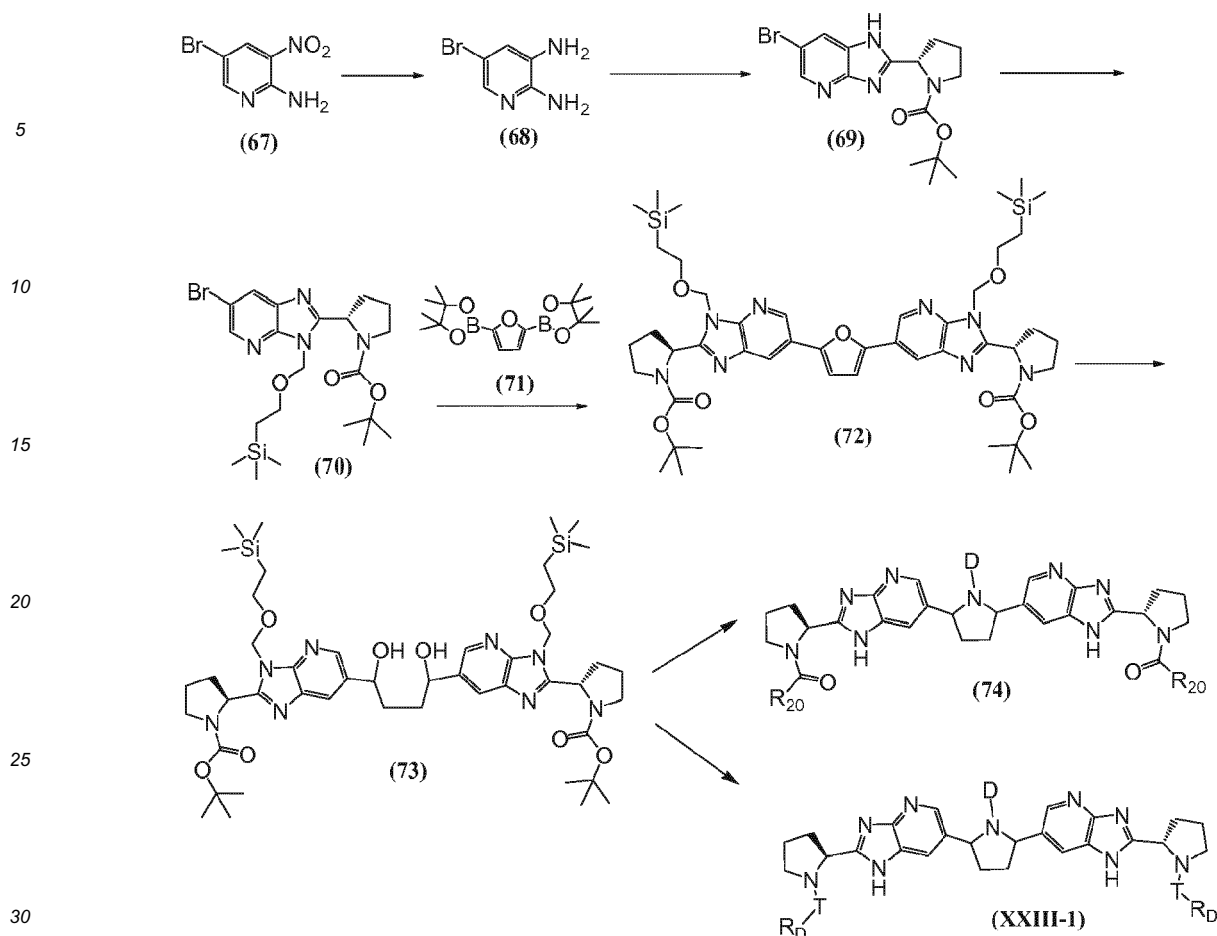
Scheme XXIII
