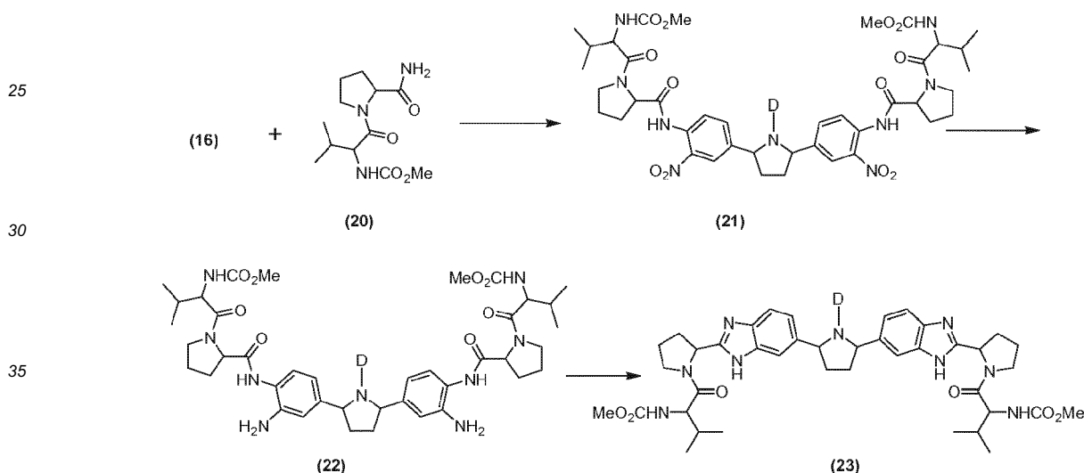
Scheme XIV
