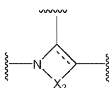
X-2
