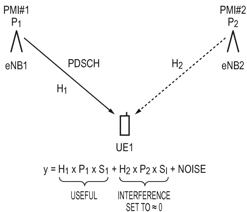
FIG. 1A (COMP + COORDINATED SCHEDULING / COORDINATED BEAMFORMING)
