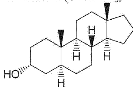
3 \alpha -Hydroxy-5 \alpha -Androstane (5 \alpha -17-dexo)
