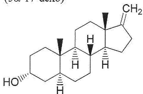
3 \alpha -Hydroxy-17-methylene- 5 \alpha -Androstane (5 \alpha -17-CH 2 )
