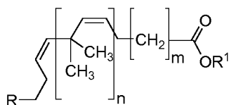
11,11-Dimethyl-octadeca-9,12-dienoic acid
