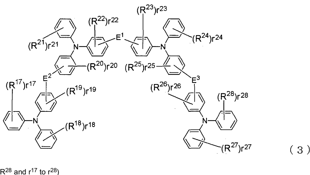
[Chemical 83]
