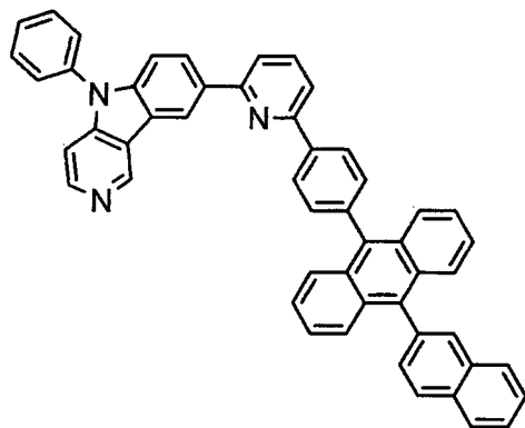
[Chemical 43]
