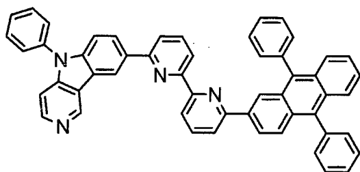
[Chemical 76]
