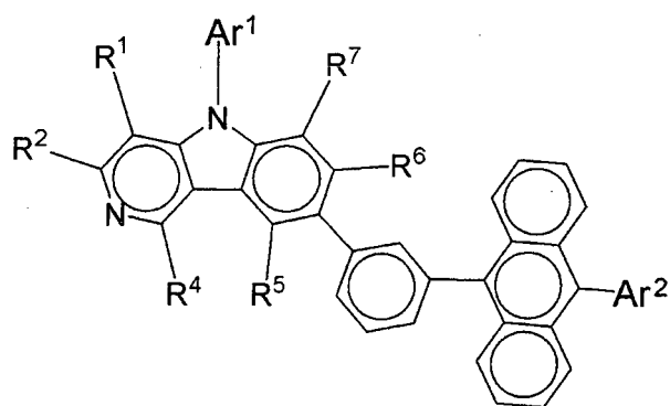
[Chemical 13]
