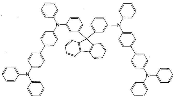
[Chemical 95]
