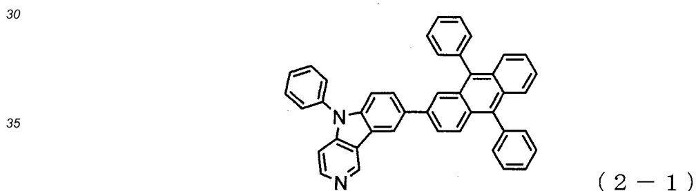
[Chemical 146]
