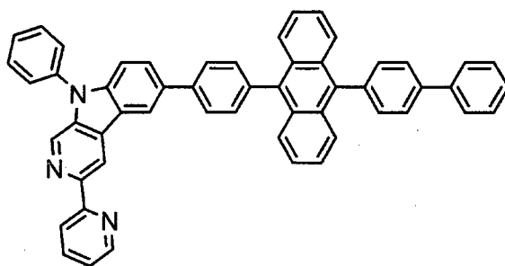
[Chemical 53]
