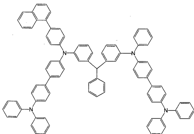
[Chemical 97]
