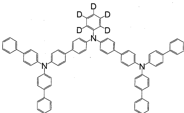
[Chemical 113]
