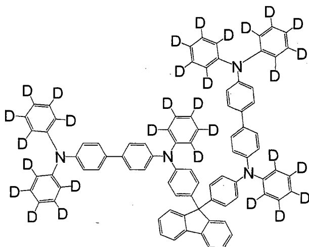
[Chemical 105]
