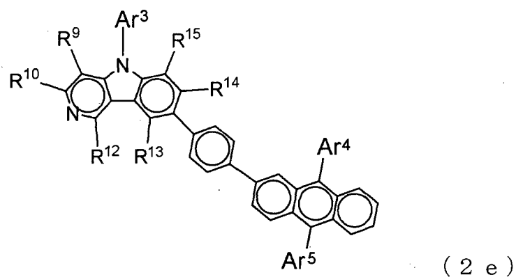
[Chemical 60]
