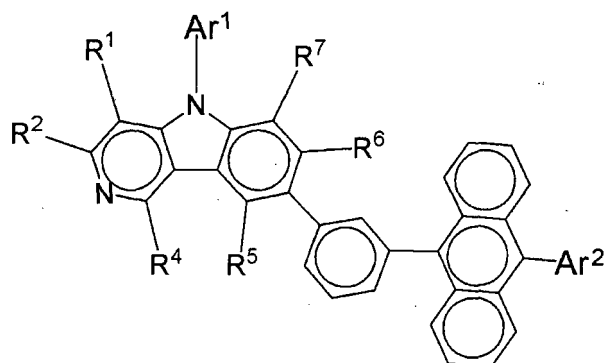
[Chemical 11]
