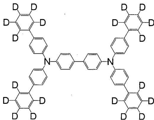
[Chemical 136]
