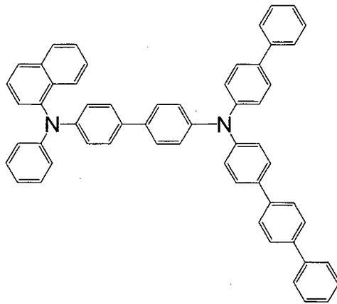
[Chemical 133]
