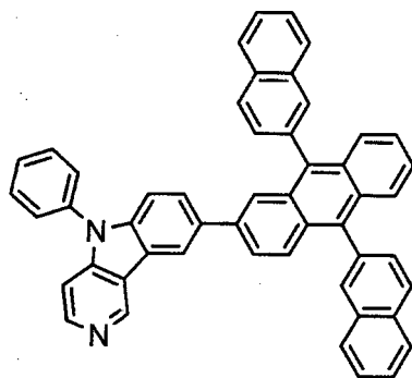
[Chemical 62]
