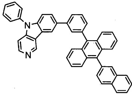
[Chemical 26]
