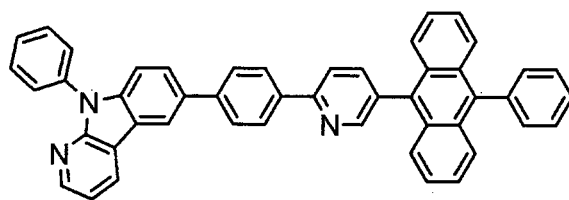
[Chemical 42]
