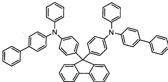
[Chemical 127]
