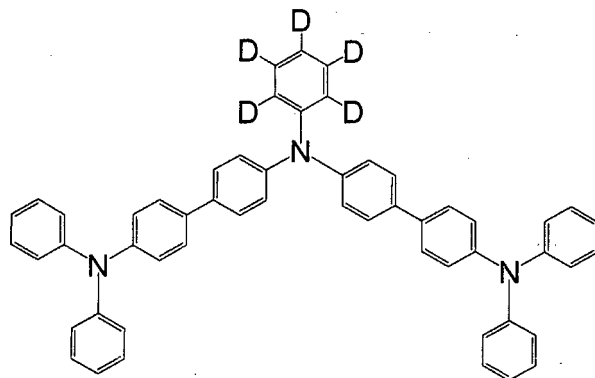
[Chemical 108]
