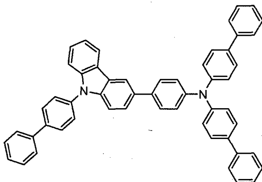
[Chemical 140]
