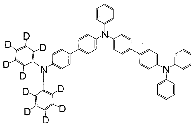
[Chemical 109]
