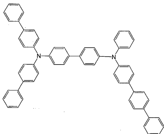
[Chemical 120]
