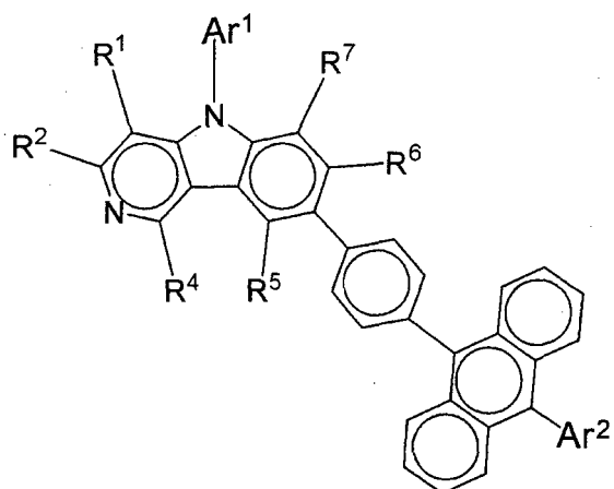
[Chemical 10]
