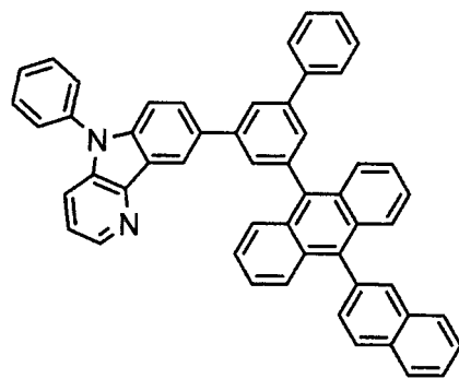
[Chemical 29]
