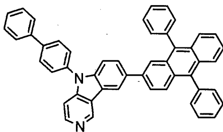
[Chemical 78]
