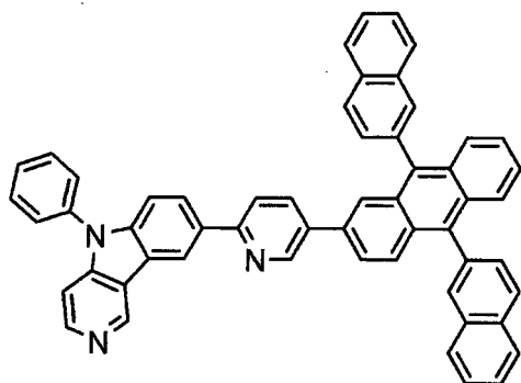
[Chemical 68]
