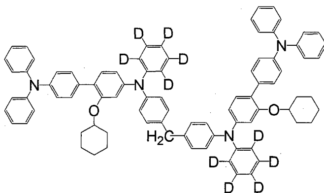
[Chemical 106]
