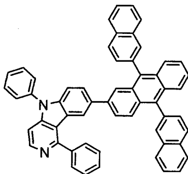
[Chemical 63]
