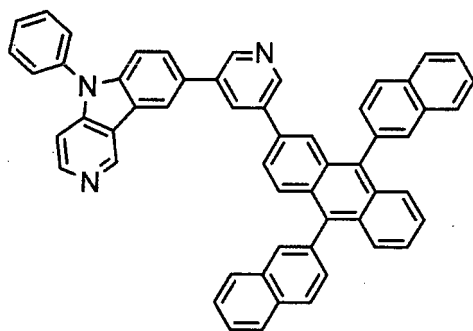
[Chemical 72]
