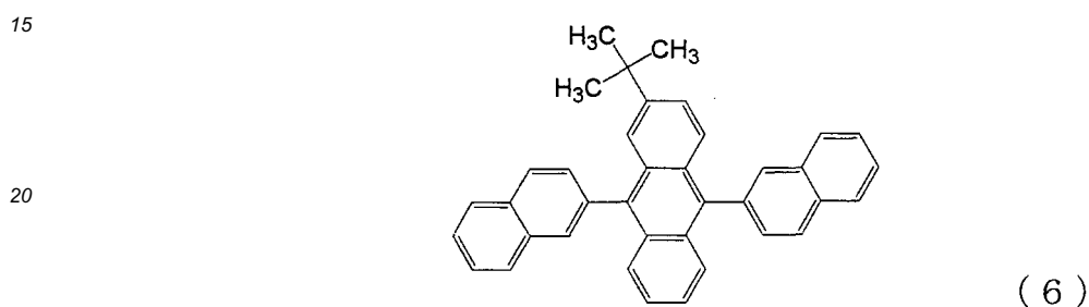
[Chemical 145]
