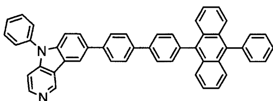
[Chemical 37]
