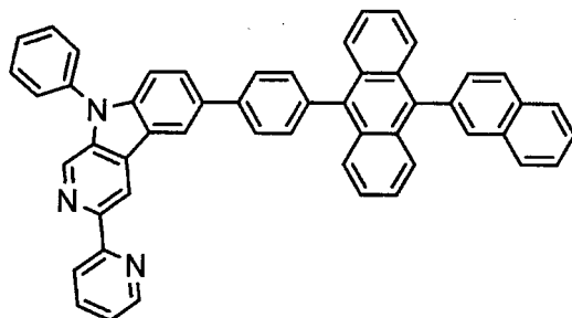
[Chemical 51]
