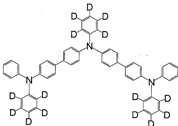
[Chemical 110]
