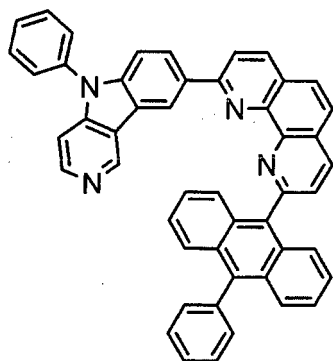
[Chemical 49]
