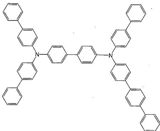
[Chemical 119]
