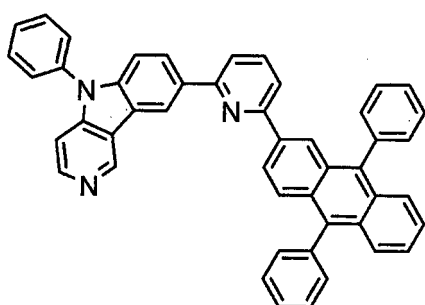
[Chemical 70]
