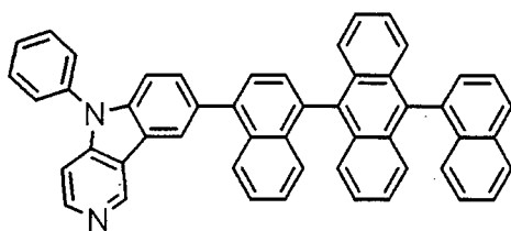
[Chemical 33]
