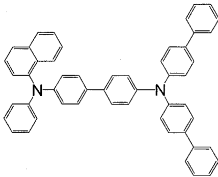
[Chemical 133]
