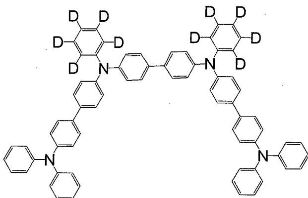
[Chemical 99]
