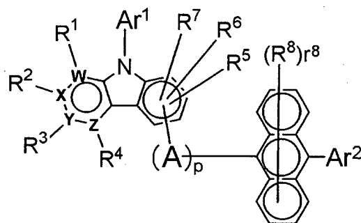
[Chemical 1]
