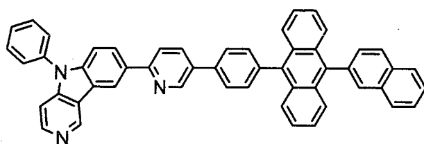
[Chemical 42]
