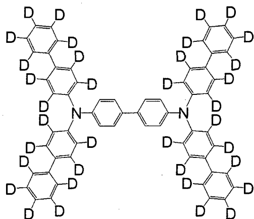
[Chemical 138]
