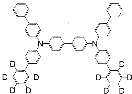
[Chemical 135]
