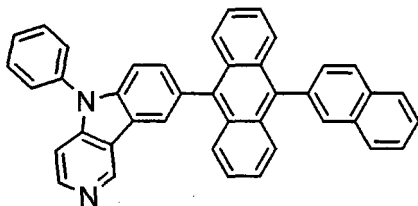
[Chemical 17]
