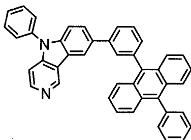
[Chemical 25]
