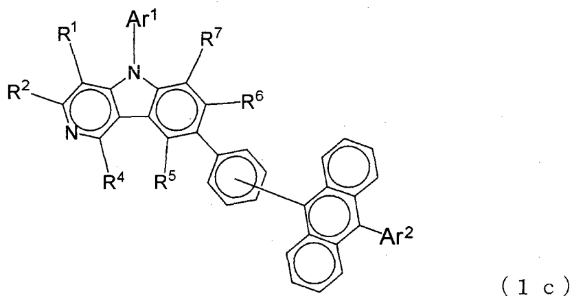
[Chemical 9]
