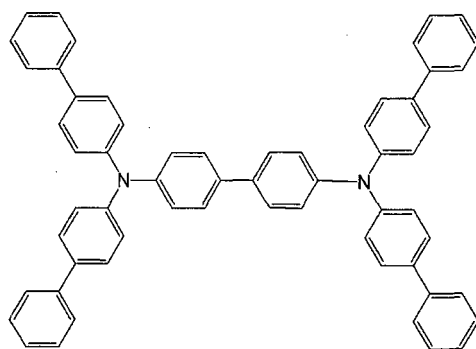
[Chemical 143]
