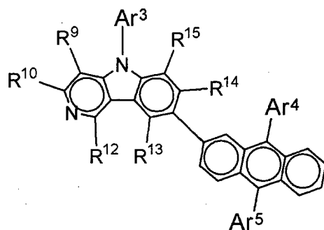
[Chemical 16]
