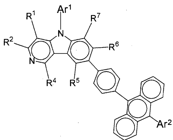
[Chemical 12]
