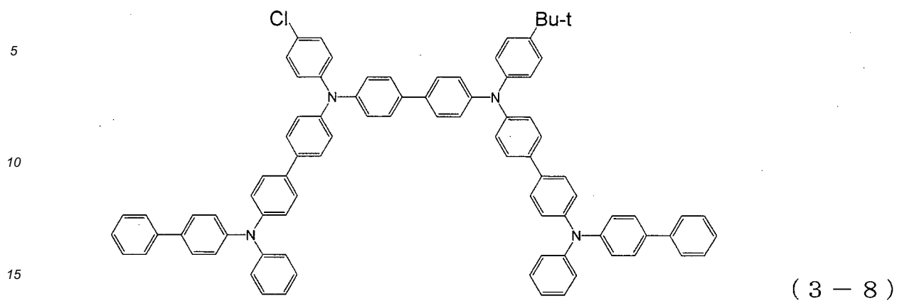
[Chemical 93]
