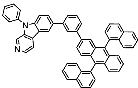
[Chemical 69]
