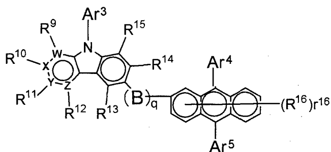
[Chemical 57]
