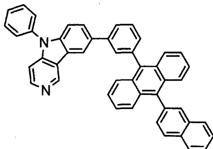
[Chemical 149]
