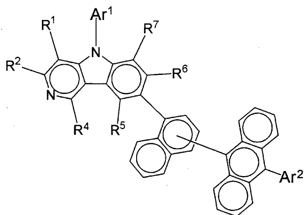
[Chemical 15]
