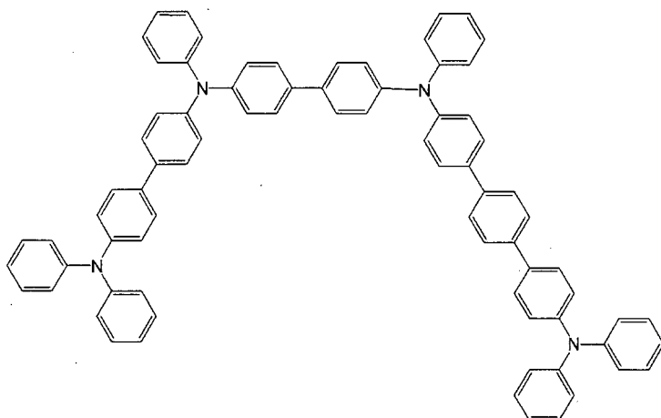
[Chemical 89]
