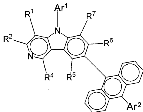
[Chemical 10]
