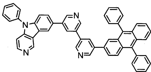
[Chemical 77]
