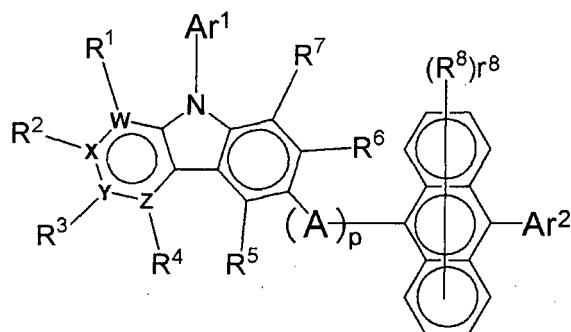
[Chemical 9]
