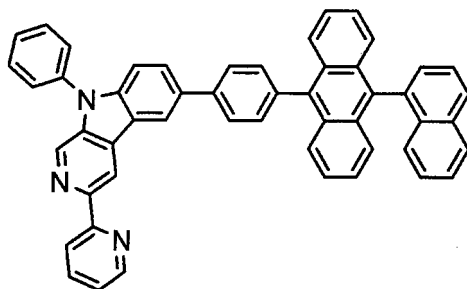
[Chemical 50]
