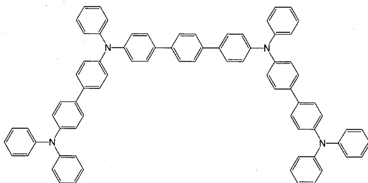
[Chemical 86]
