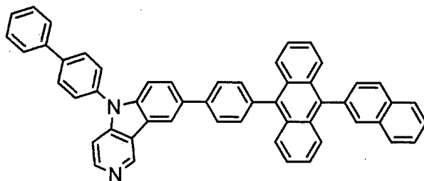
[Chemical 24]
