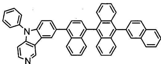
[Chemical 34]
