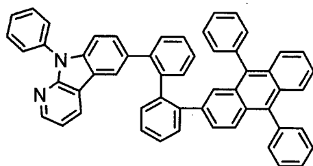
[Chemical 74]
