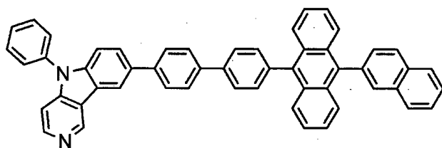
[Chemical 38]
