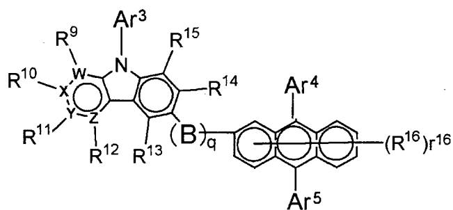
[Chemical 15]
