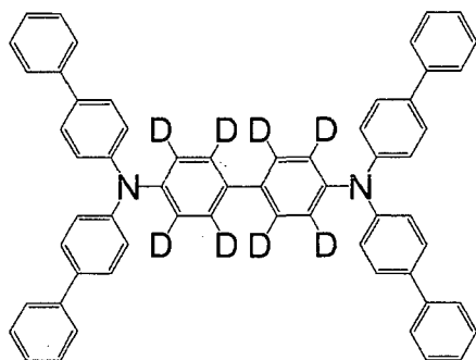
[Chemical 137]
