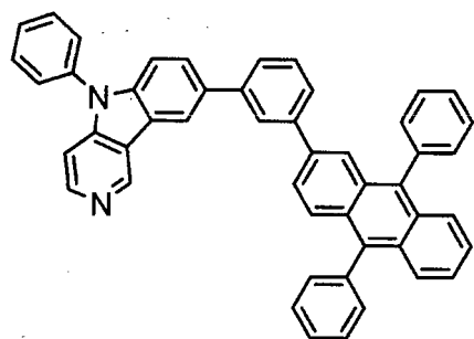
[Chemical 68]
