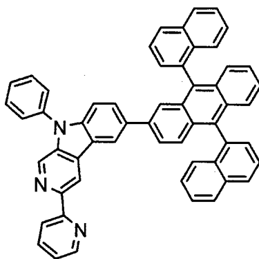
[Chemical 80]
