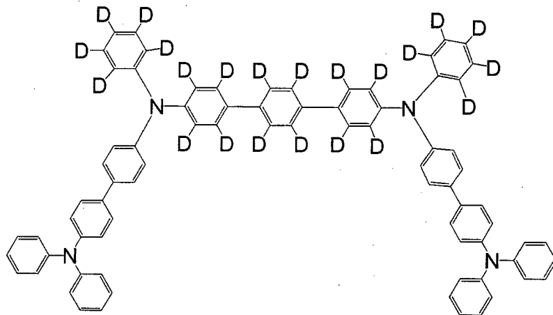
[Chemical 103]
