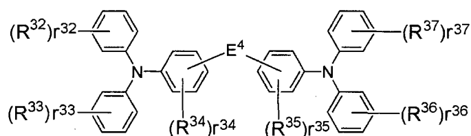
[Chemical 115]
