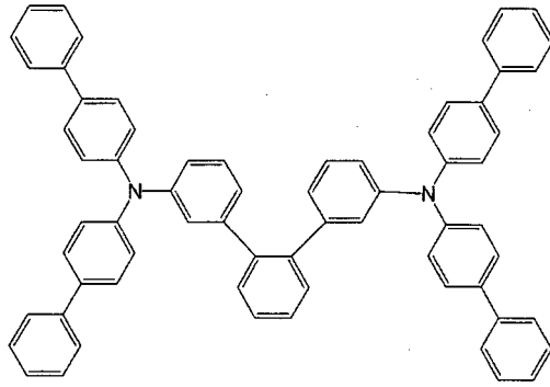
[Chemical 125]
