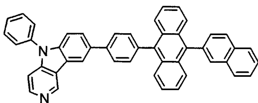
[Chemical 22]
