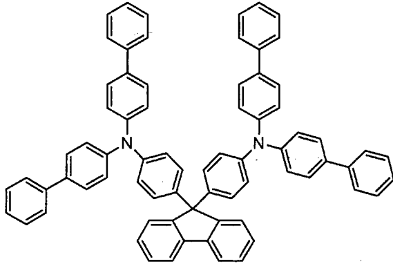
[Chemical 132]
