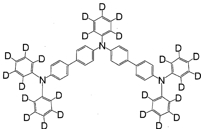
[Chemical 111]
