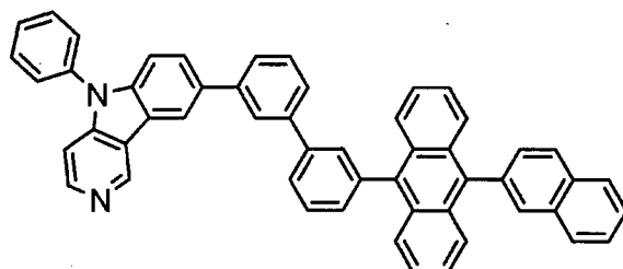
[Chemical 39]
