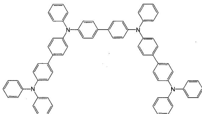
[Chemical 142]
