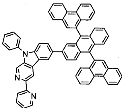
[Chemical 81]
