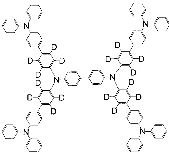
[Chemical 100]
