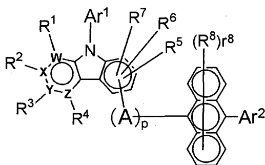
[Chemical 7]
