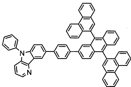
[Chemical 66]
