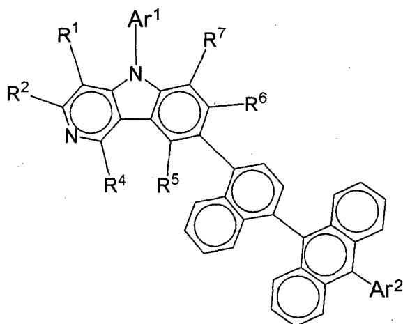
[Chemical 13]
