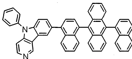
[Chemical 151]
