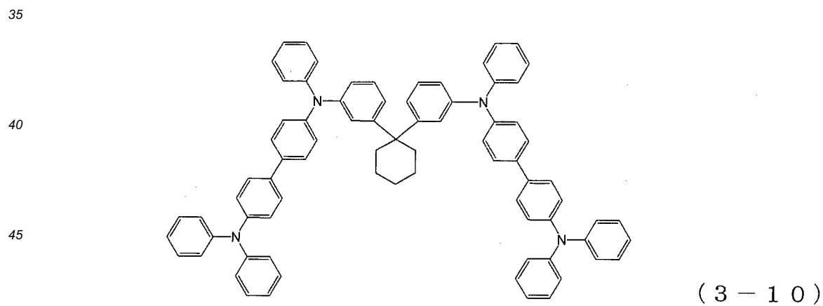
[Chemical 94]
