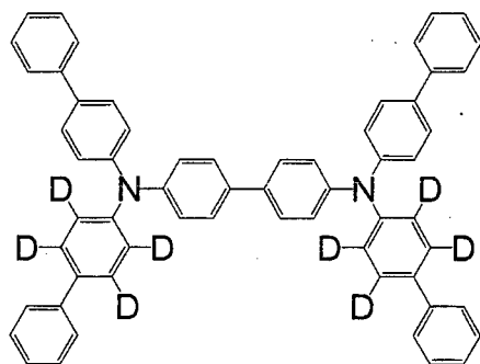
[Chemical 135]
