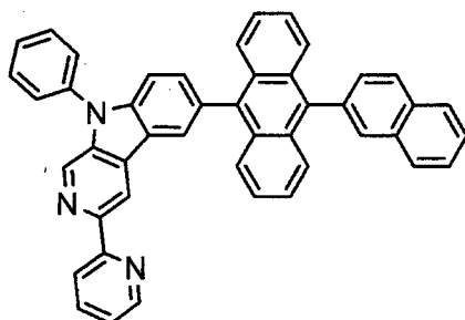
[Chemical 54]
