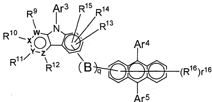
[Chemical 8]
