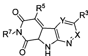
(I-d)
