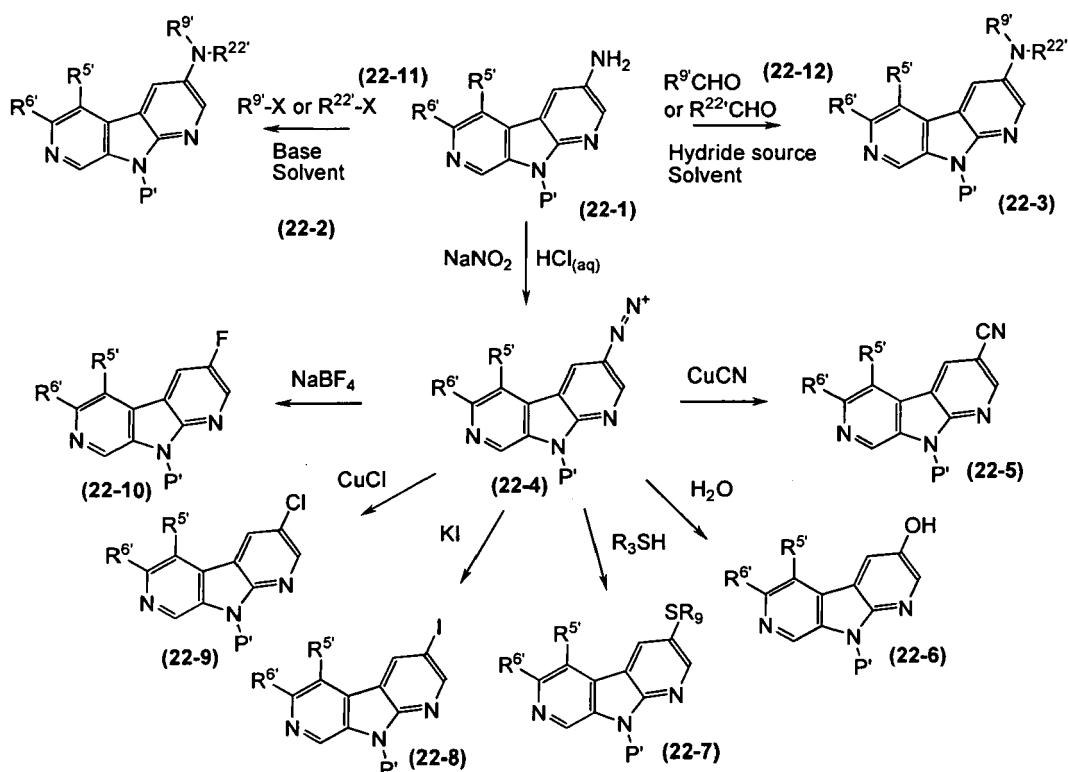
Scheme 22
