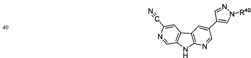
45 Formula III
