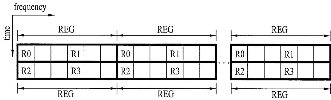
(b) 4 TX
