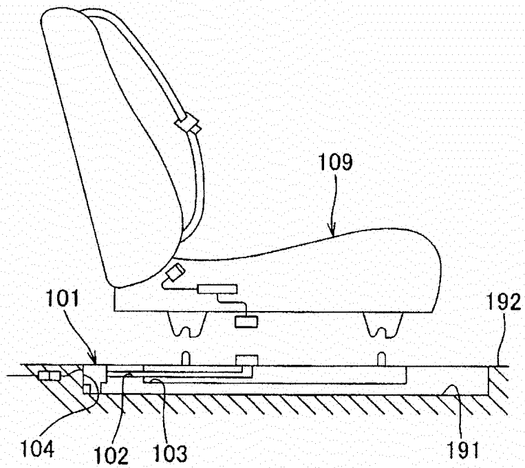
FIG. 12 PRIOR ART
