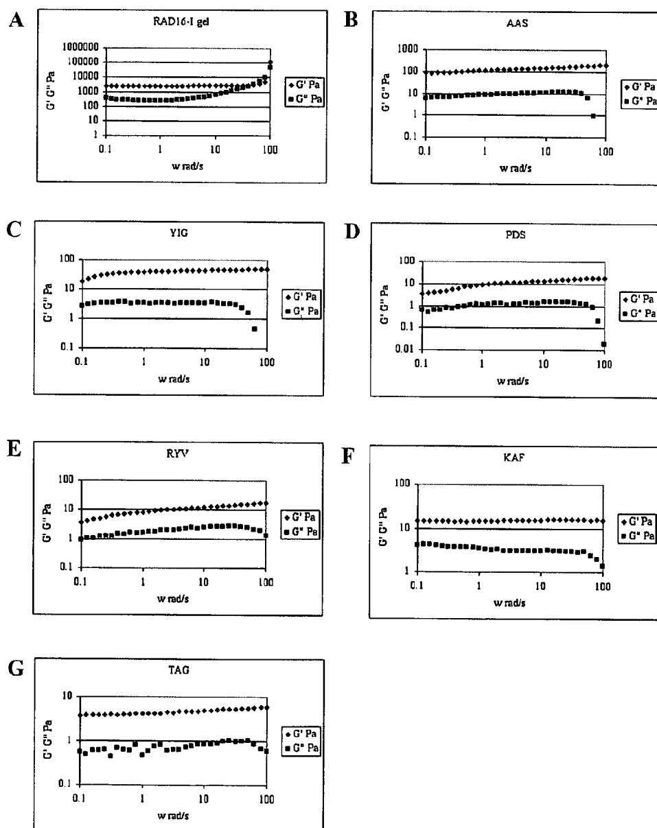
Figure 6. Dynamic frequency sweep test for peptide scaffolds at a fixed strain=0.01. A) RAD16-I, B) AAS, C) YIG, D) PDS, E) RYV, F) KAF, G) TAG. G' (Storage modulus) represents the elastic character of the material, and G'' (Loss modulus) represents its viscous character.
