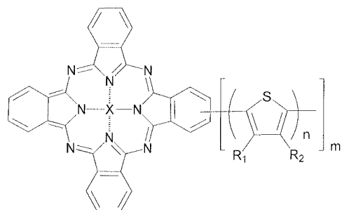
[Chem. 13]
