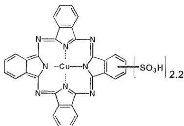
[Chem. 7]
