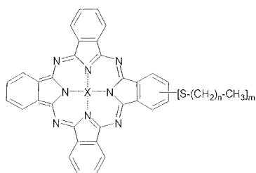
[Chem. 11]
