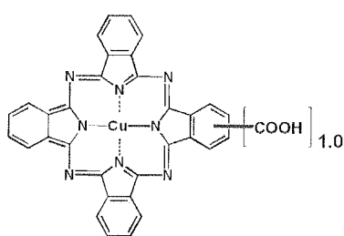
[Chem. 8]
