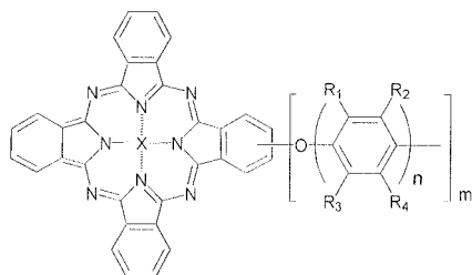
[Chem. 12]
