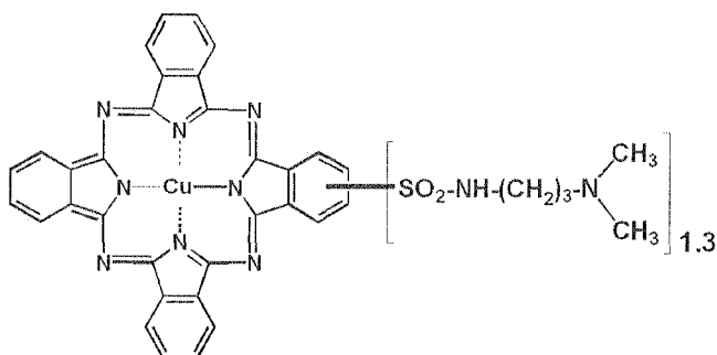
[Chem. 18]
