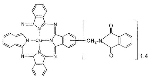
[Chem. 10]
