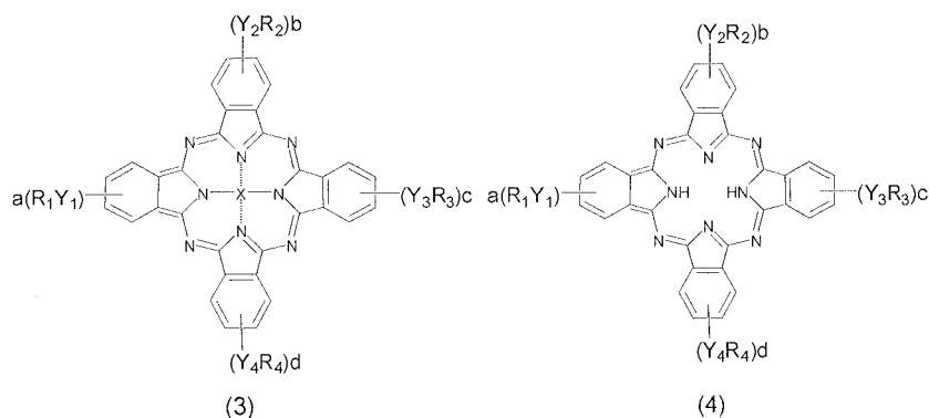
[Chem. 2]
