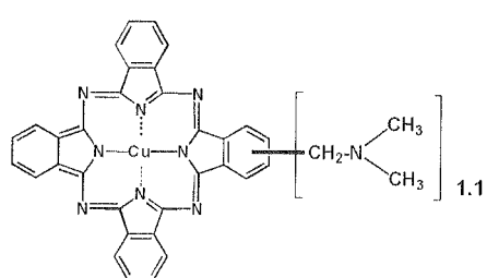
[Chem. 9]
