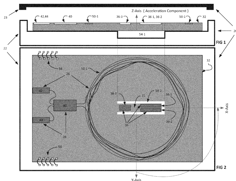
Coaxial Gyro Accelerometer in a Semiconductor Substrate
