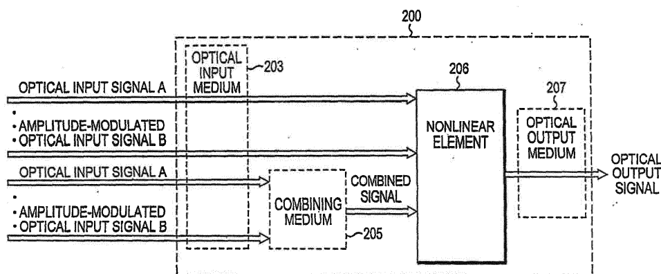
GENERALIZED ALL-OPTICAL LOGICAL GATE
