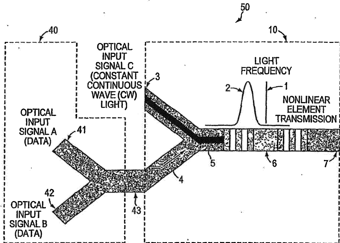
ALL-OPTICAL NOR GATE RECEIVING ONE OR TWO 1-BITS AND OUTPUTTING A 0-BIT
