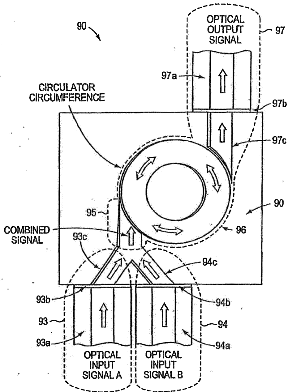
ALL-OPTICAL LOGICAL GATE USING COMBINING MEDIUM AND RESONATOR IMPLEMENTED AS A CIRCULATOR
