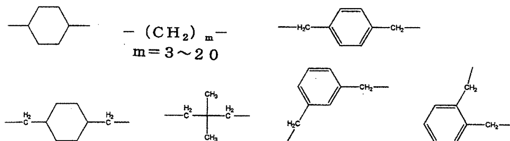
[Chemical Formula 13]
