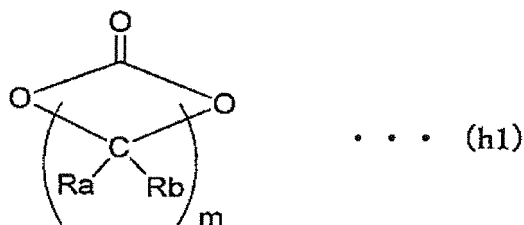
[Chemical Formula 14]
