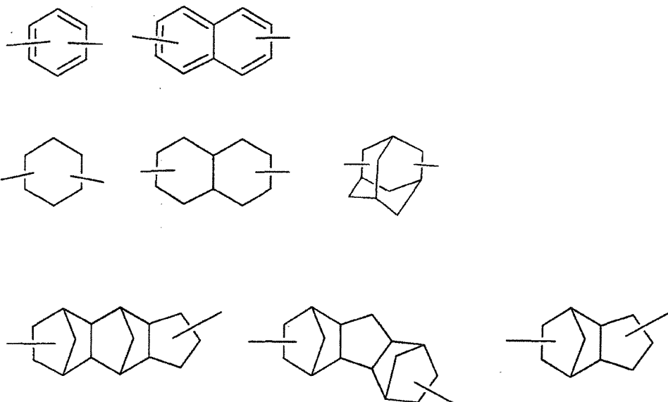
[Chemical Formula 49]
