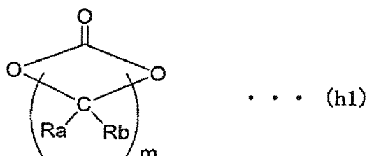
[Chemical Formula 17]
