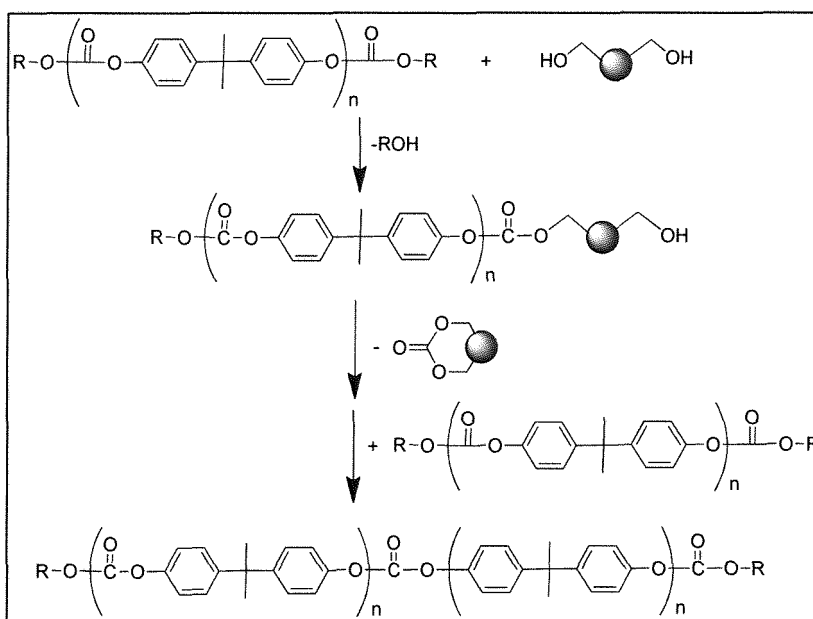
[Chemical Formula 74]
