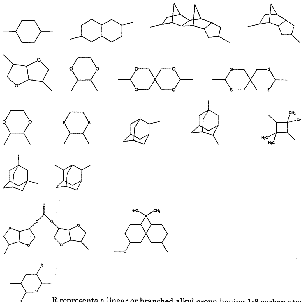
[Chemical Formula 34]
