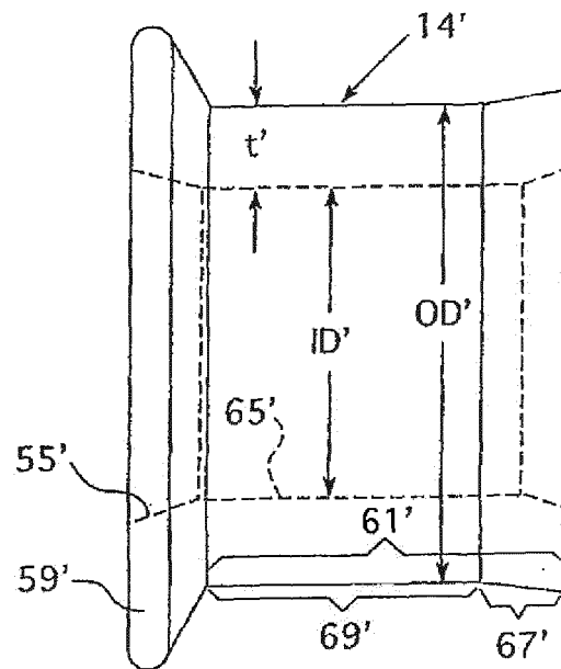
FIG. 4 Prior Art
