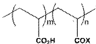
Fluorescein tagged PAA (PAA-F)
