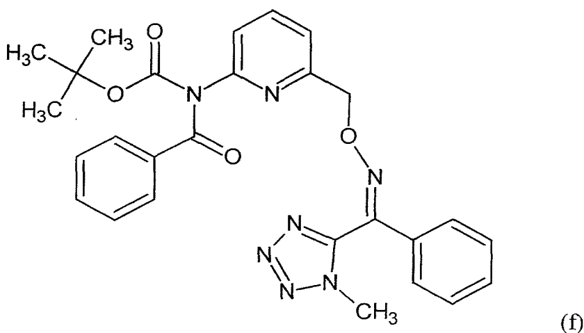
[Chemical Formula 19]
