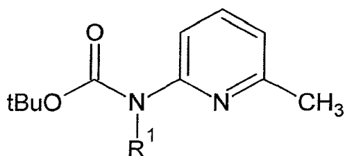
[Chemical Formula 14]
