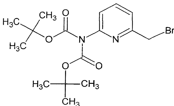
[Chemical Formula 25]
