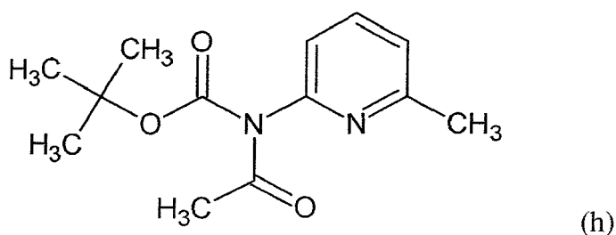
[Chemical Formula 21]
