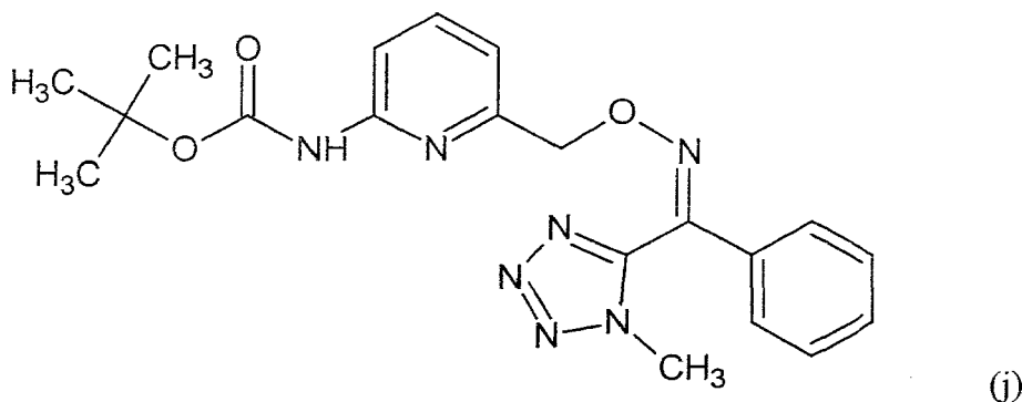
[Chemical Formula 23]
