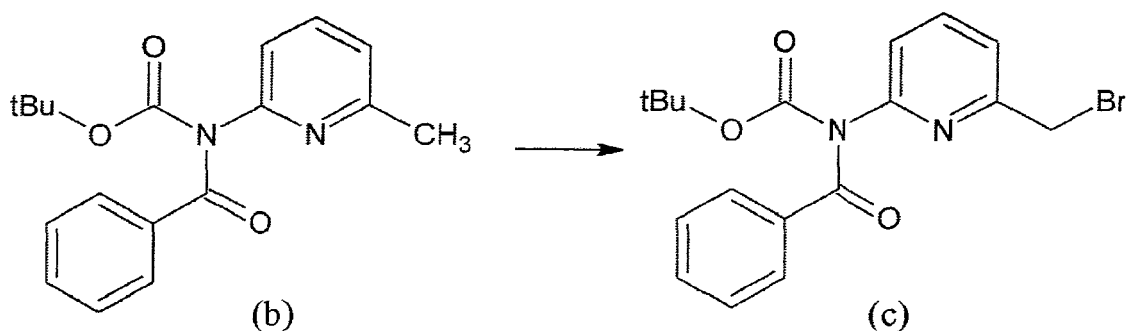
[Chemical Formula 13]
