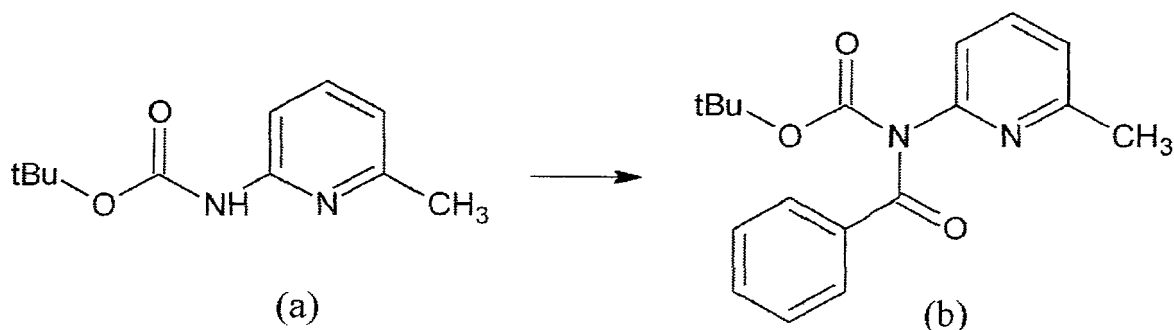
[Chemical Formula 12]
