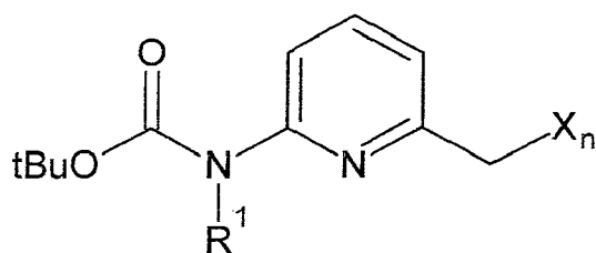
[Chemical Formula 15]
