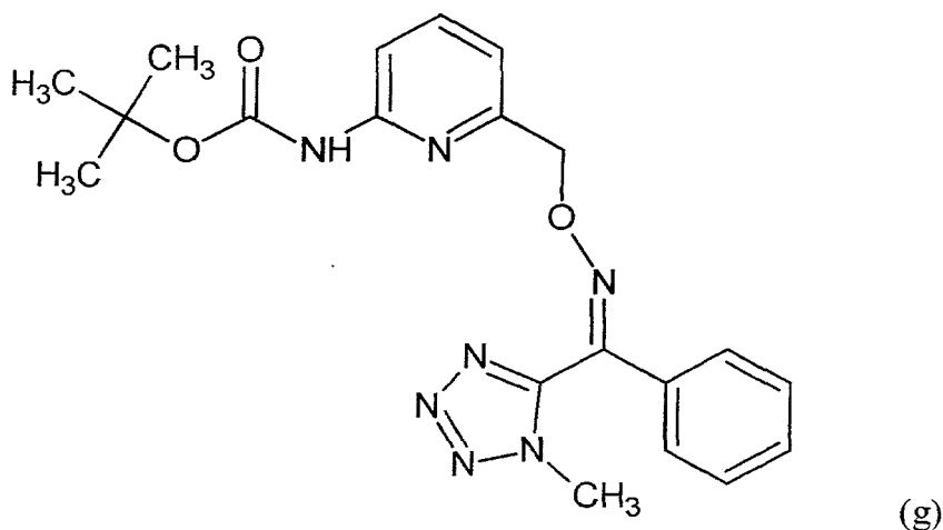
[Chemical Formula 20]
