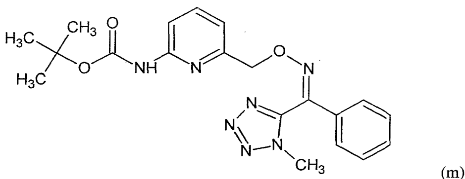
[Chemical Formula 26]
