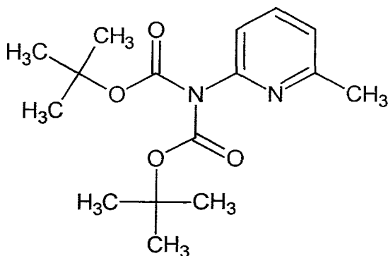
[Chemical Formula 24]
