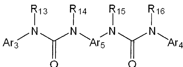
Structural Formula (5)
