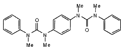
Exemplified Compound (2-5)
