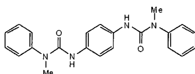
Exemplified Compound (2-10)
