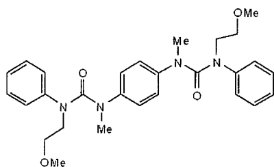
Exemplified Compound (2-7)
