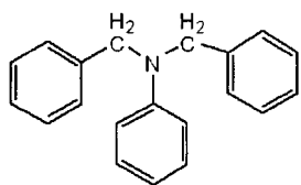
Exemplified Compound (1-1)
