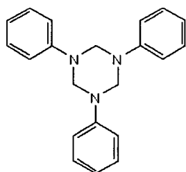
Exemplified Compound (1-6)
