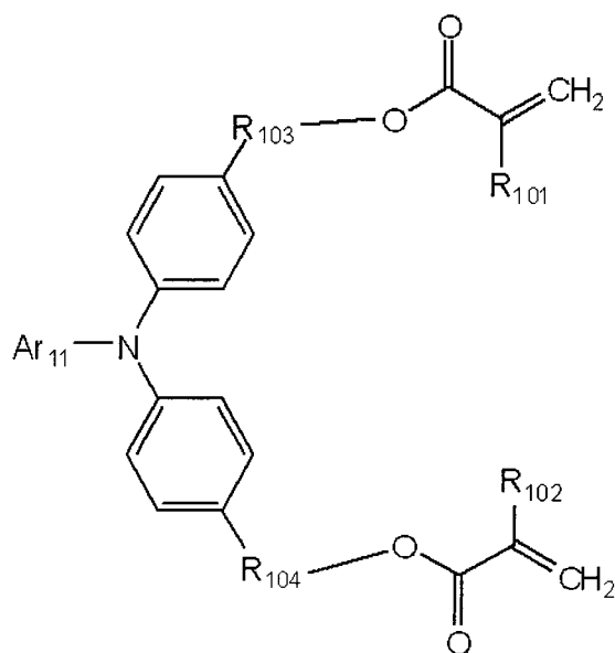
Structural Formula (6)
