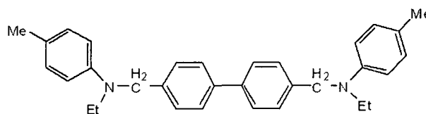
Exemplified Compound (1-5)
