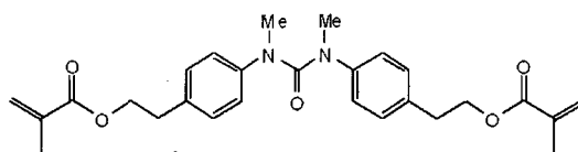
Exemplified Compound (2-12)
