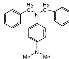
Exemplified Compound (1-3)
