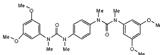
Exemplified Compound (2-9)
