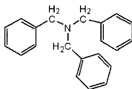
Exemplified Compound (1-2)
