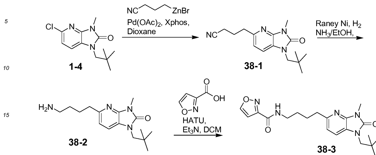
Scheme 38
