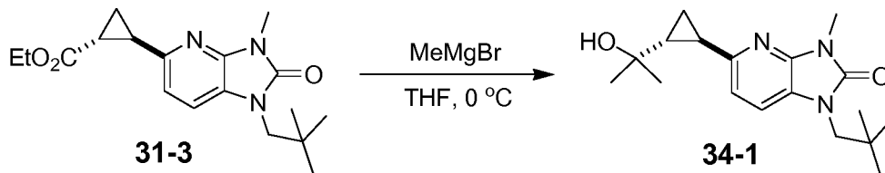
Scheme 34
