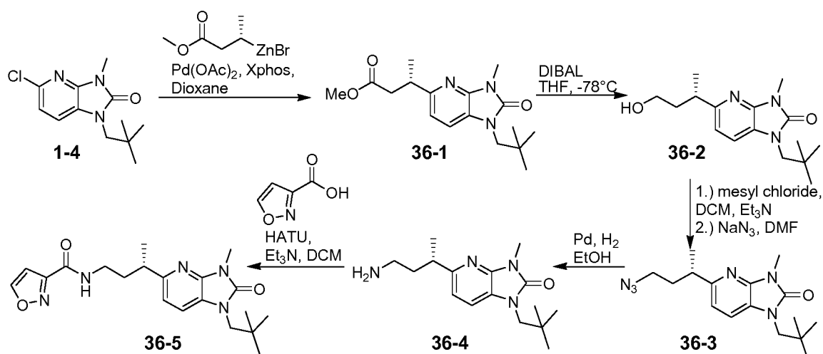
Scheme 36
