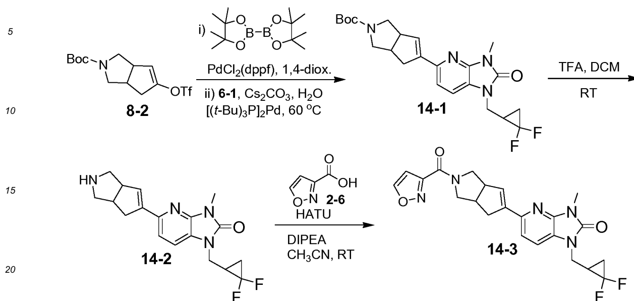
Scheme 14
