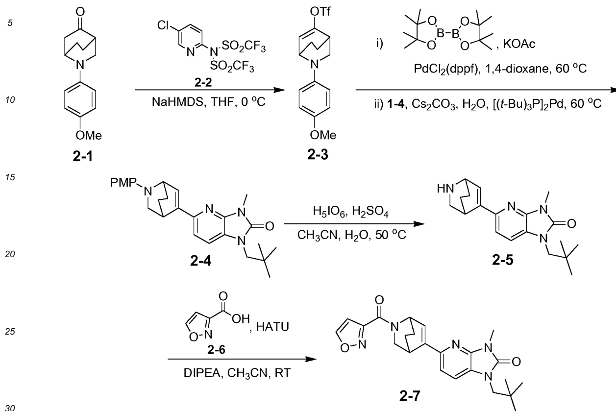
Scheme 2
