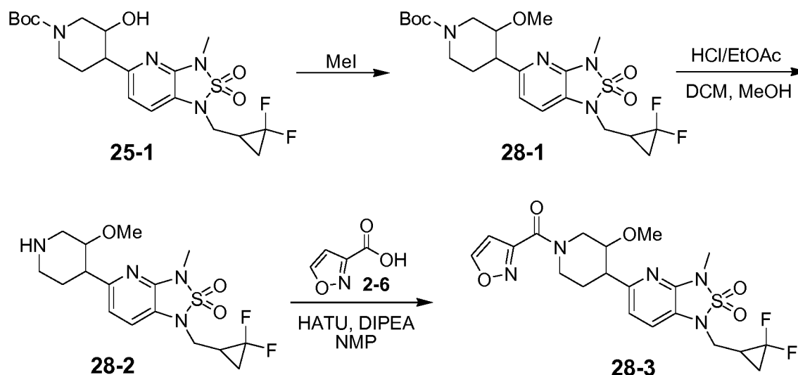
Scheme 28 (illustrative)
