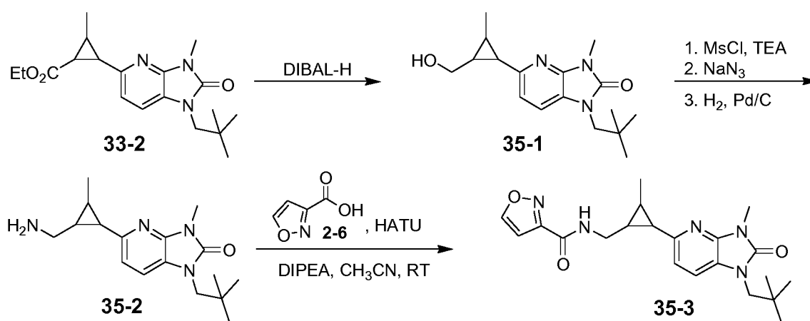
Scheme 35
