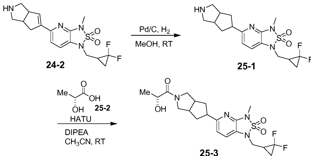
Scheme 25 (illustrative)
