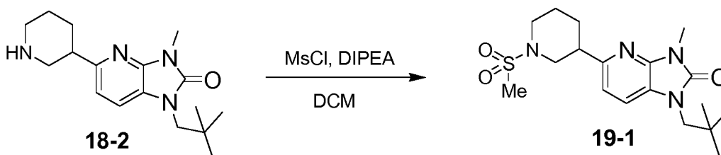
Scheme 19
