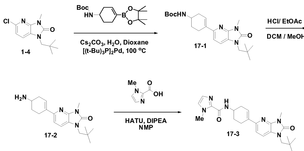
Scheme 17
