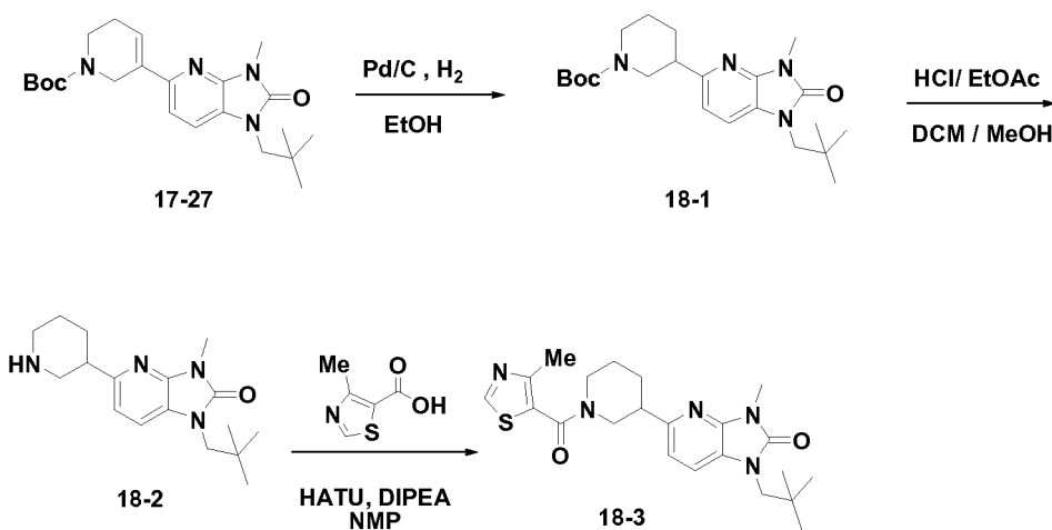
Scheme 18
