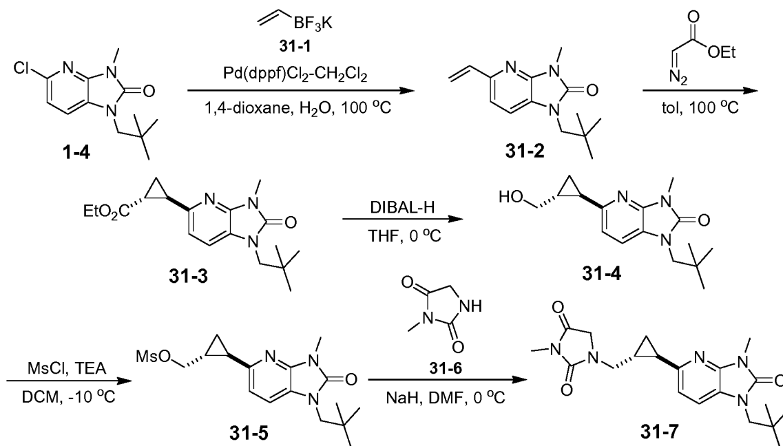
Scheme 31
