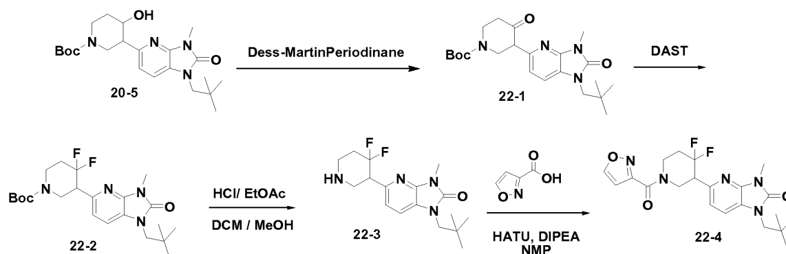
Scheme 22
