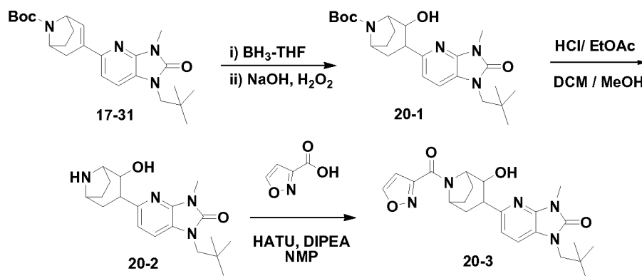
Scheme 20
