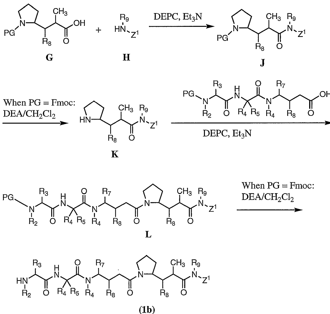
Scheme 6
