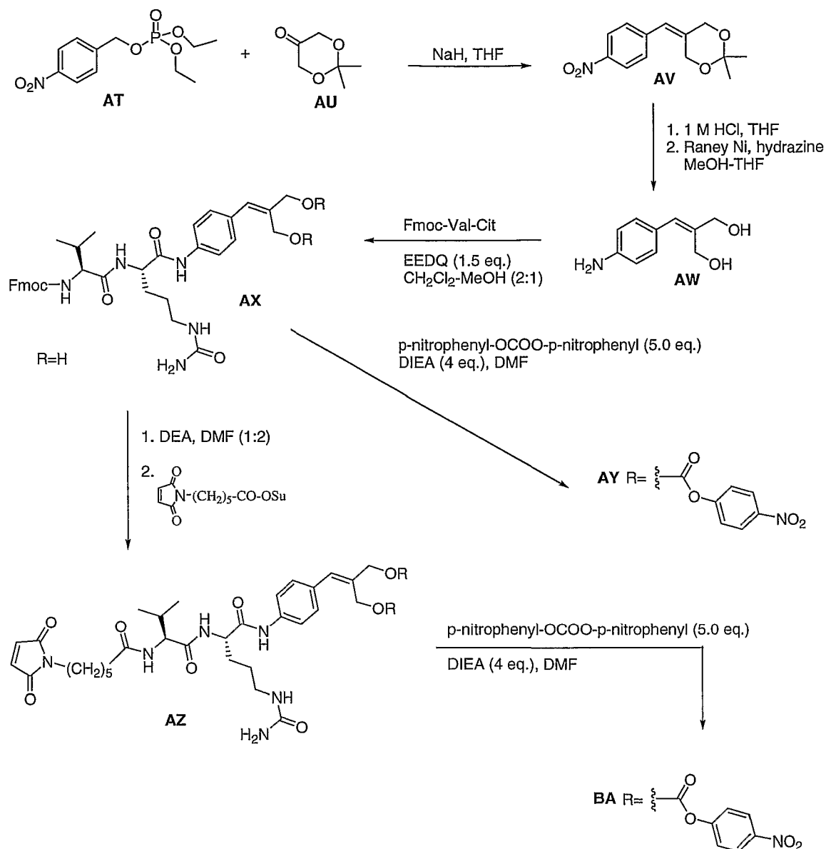
Scheme 15
