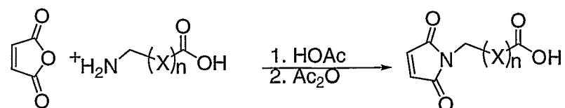
Scheme 8
