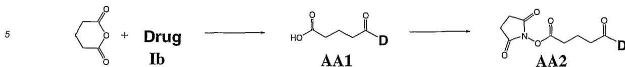
Scheme 13a
