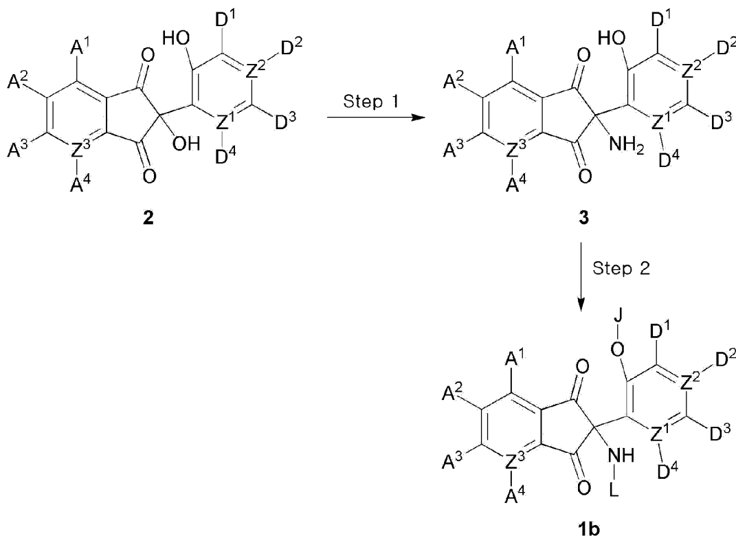
[Reaction Scheme 2]
