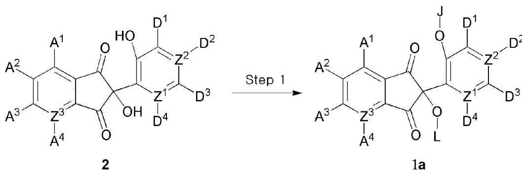
[Reaction Scheme 1]
