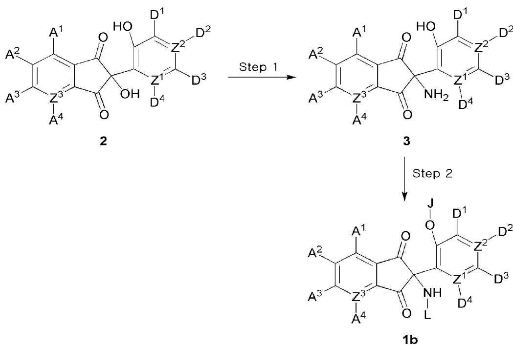
[Reaction Formula 2]
