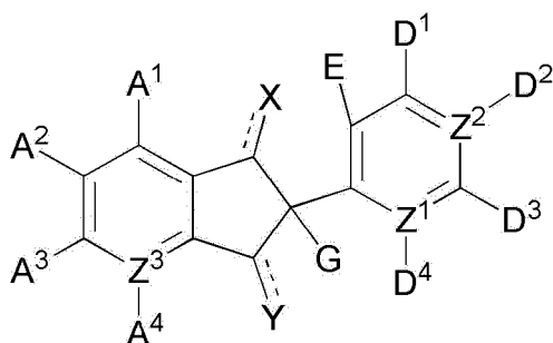
[Chemical Formula 1]
