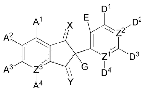
[Chemical Formula 1]
