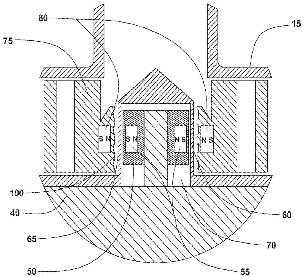
FIG 4 (DETAIL C)
