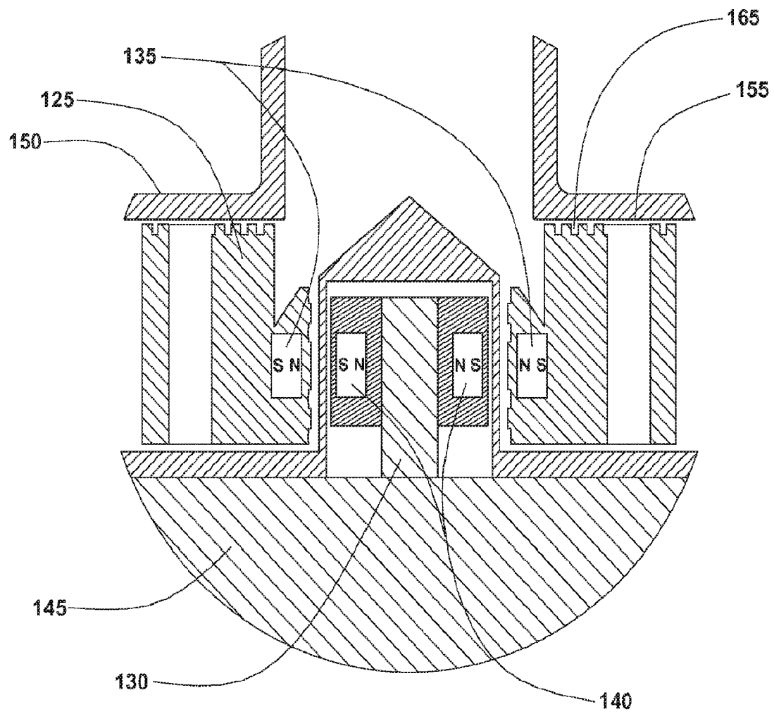
FIG. 13 (DETAIL D)
