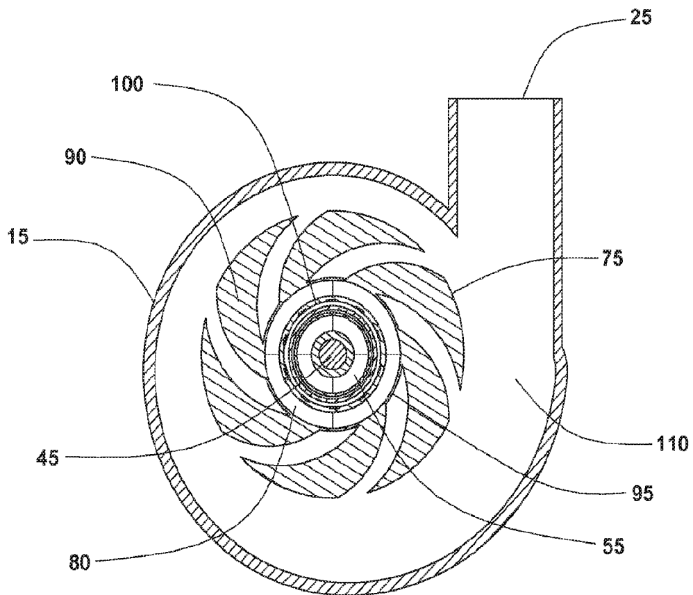
FIG. 3 (SECTION B - B)
