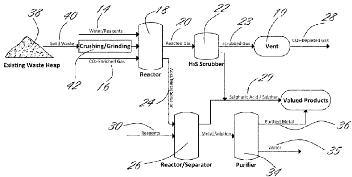
Figure 2: Reprocessing Solid Material
