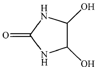
4,5-dihydroxyimidazolidin-2-one
