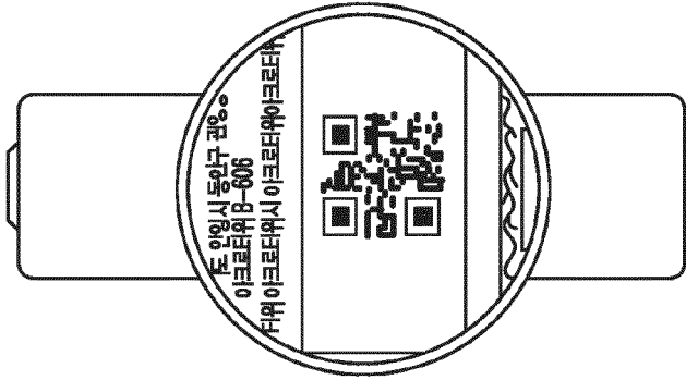
BARCODE RECOGNITION
