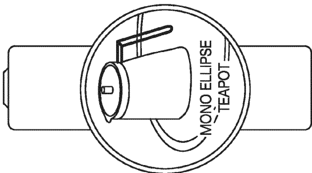
OBJECT RECOGNITION
