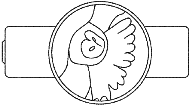
IMAGE RECOGNITION
