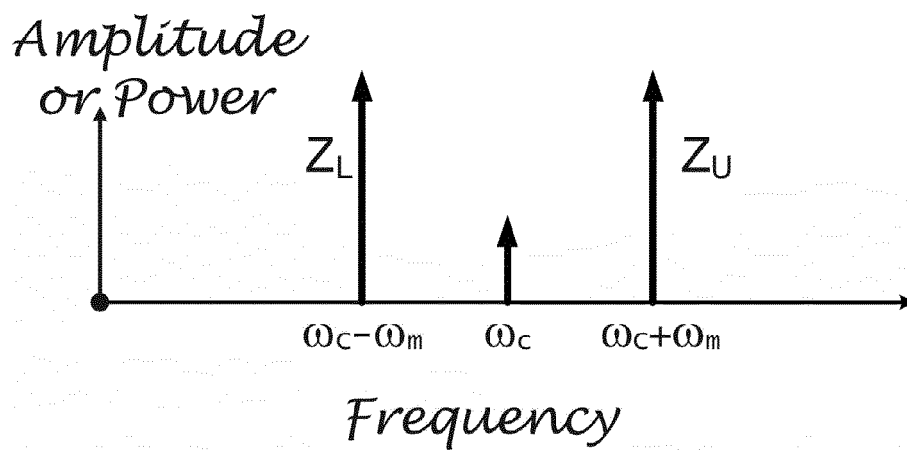
FIGURE 2 (Conventional)
