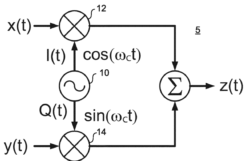
FIGURE 1 (Conventional)
