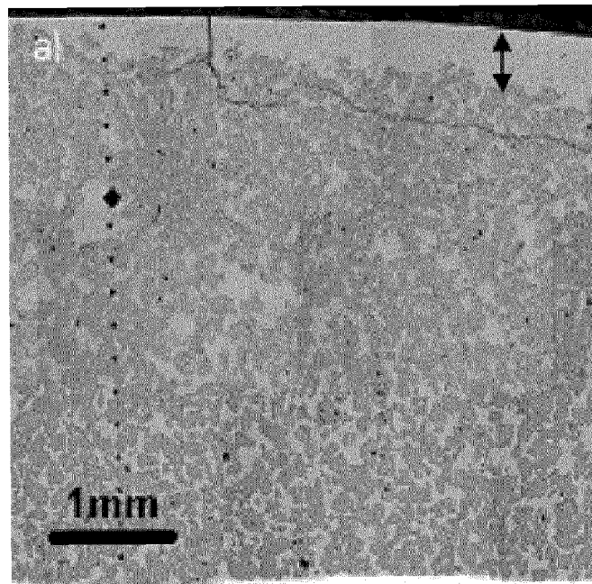
Figure 8 (Prior Art)
