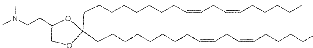
DLin-K-C2-DMA
