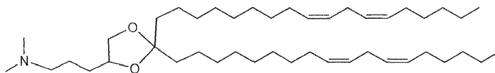
DLin-K-C3-DMA; or
