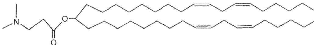
DLin-M-K-DMA; or
