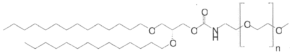
PEG-C-DOMG
