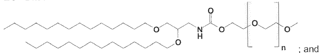
PEG- DMA
