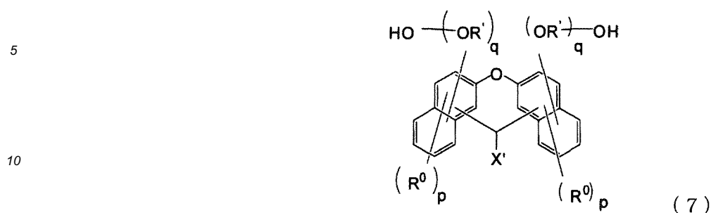
[Chemical Formula 77]
