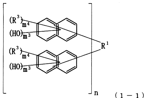
[Chemical Formula 18]
