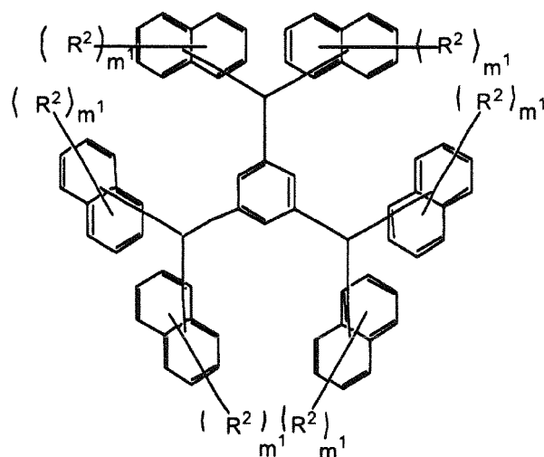
[Chemical Formula 25]
