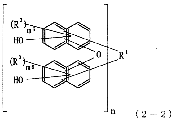
[Chemical Formula 6]
