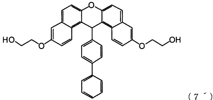
[Chemical Formula 84]
