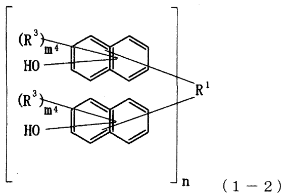
[Chemical Formula 5]
