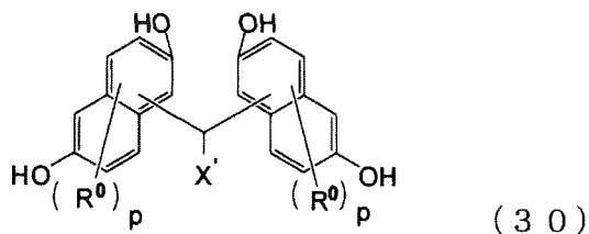
[Chemical Formula 14]
