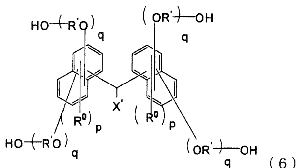
[Chemical Formula 14]
