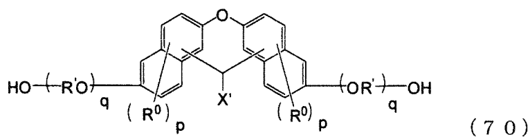
[Chemical Formula 16]
