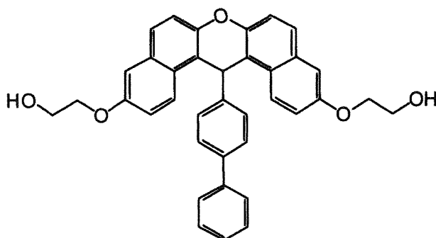
[Chemical Formula 116]
