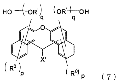
[Chemical Formula 14]
