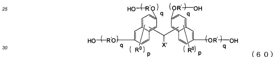
[Chemical Formula 79]
