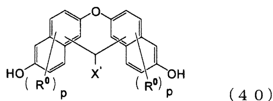
[Chemical Formula 14]
