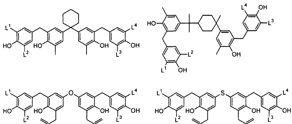
[Chemical Formula 62]
