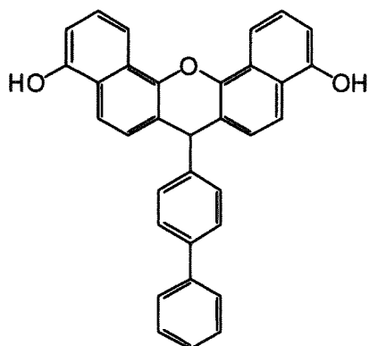
(XBisN-3)
