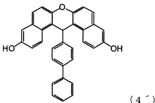
[Chemical Formula 84]
