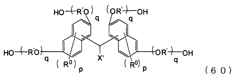
[Chemical Formula 21]
