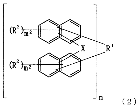
[Chemical Formula 2]
