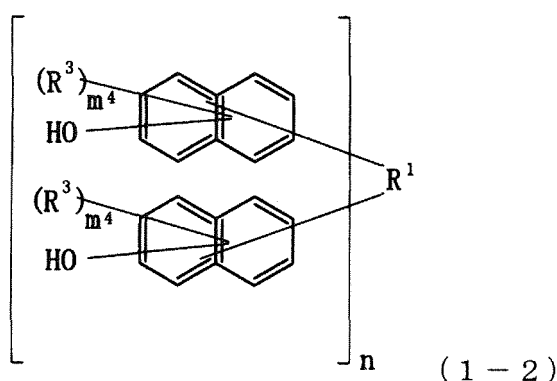
[Chemical Formula 19]
