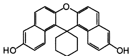
(XBisN-10)
