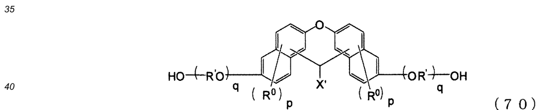
[Chemical Formula 79]
