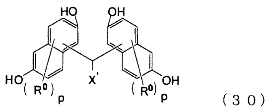
[Chemical Formula 12]
