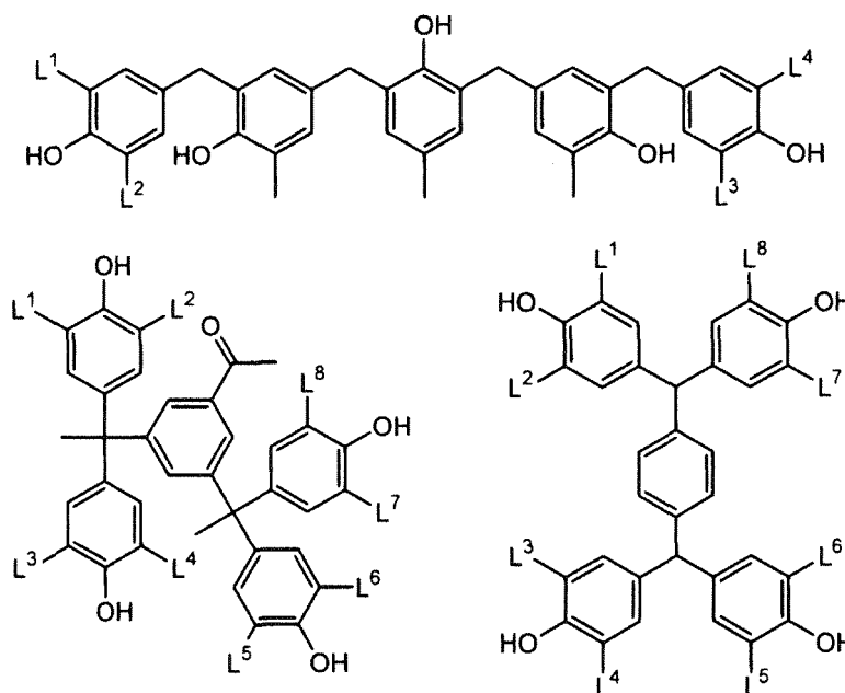
[Chemical Formula 63]
