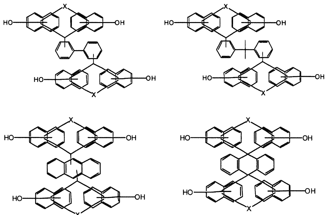
[Chemical Formula 45]
