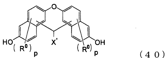
[Chemical Formula 10]
