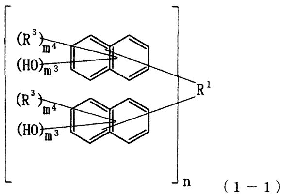
[Chemical Formula 3]
