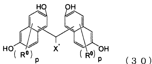
[Chemical Formula 10]
