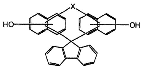
[Chemical Formula 43]
