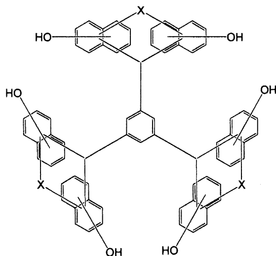
[Chemical Formula 45]
