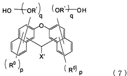
[Chemical Formula 18]
