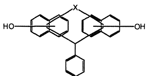
[Chemical Formula 41]
