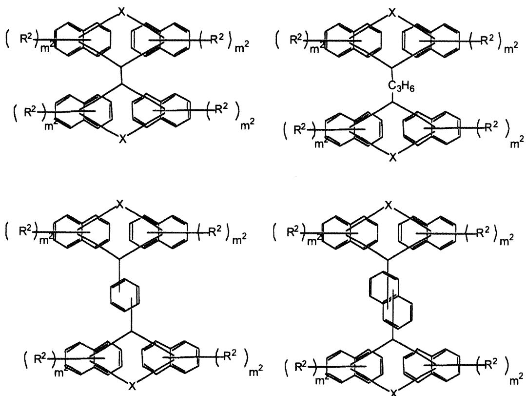
[Chemical Formula 39]
