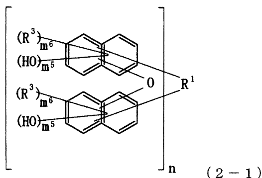
[Chemical Formula 32]
