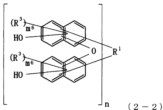
[Chemical Formula 6]
