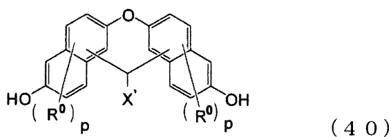
[Chemical Formula 12]
