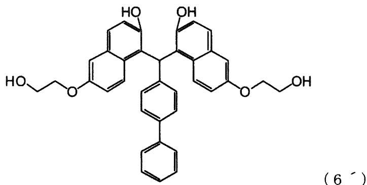
[Chemical Formula 81]
