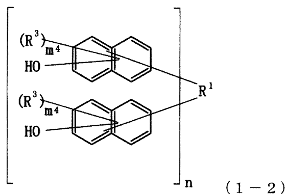
[Chemical Formula 6]
