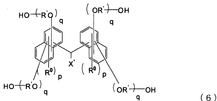
[Chemical Formula 19]
