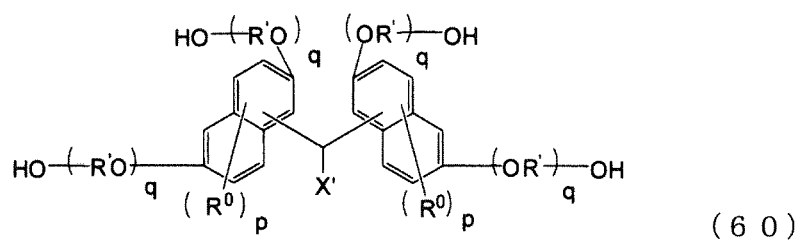
[Chemical Formula 16]
