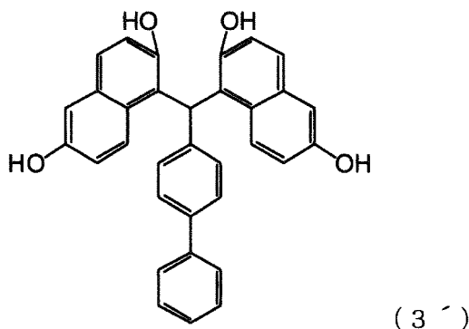
[Chemical Formula 81]
