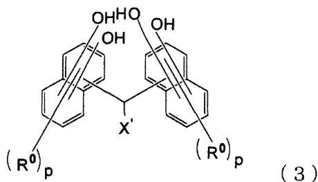
[Chemical Formula 7]
