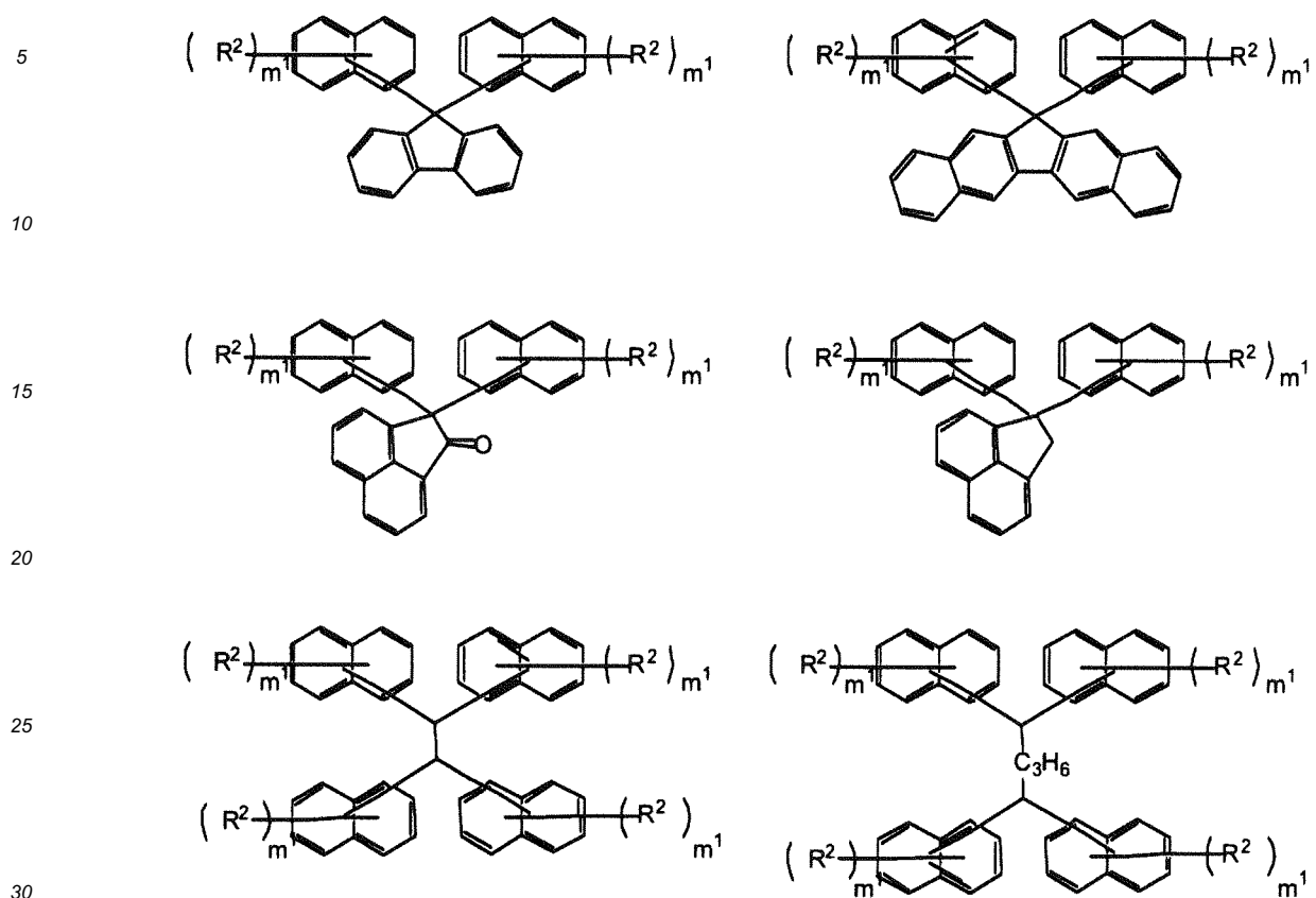
[Chemical Formula 24]
