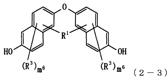
[Chemical Formula 34]
