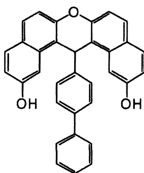
(XBisN-2)
