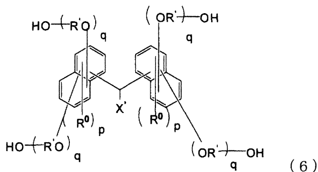
[Chemical Formula 18]
