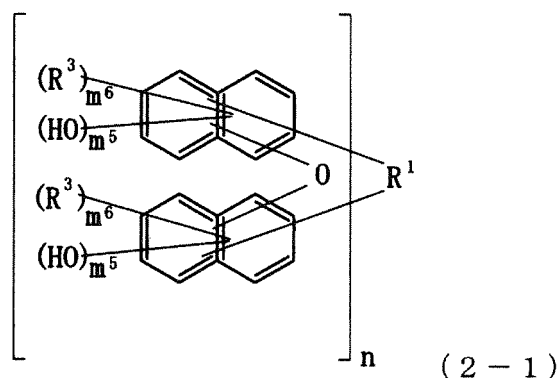
[Chemical Formula 4]
