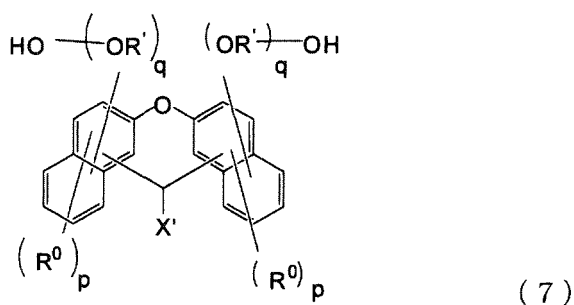
[Chemical Formula 20]
