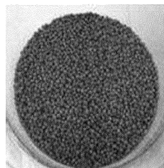
CuBTC Composite
