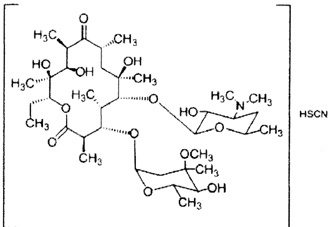
Formula I
