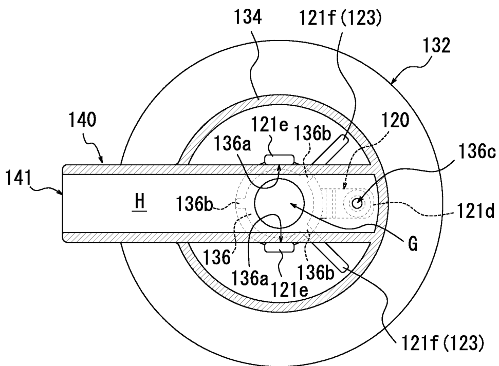
D-D Sectional View
