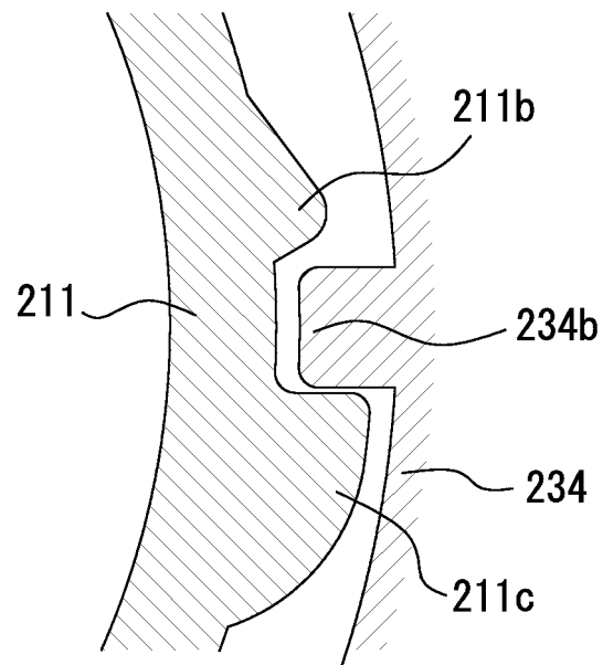
C-C Sectional View
