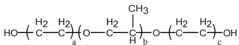
Structure of Pluronic F127.
