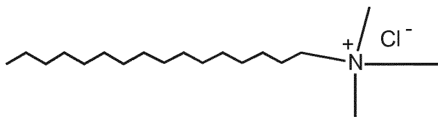
Structure of cetyltrimethylammonium chloride (CTAC).
