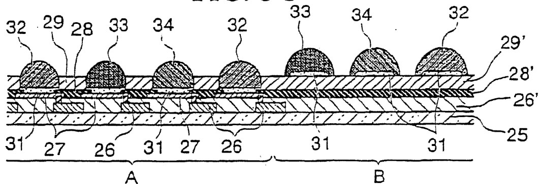
FIG. 3D
